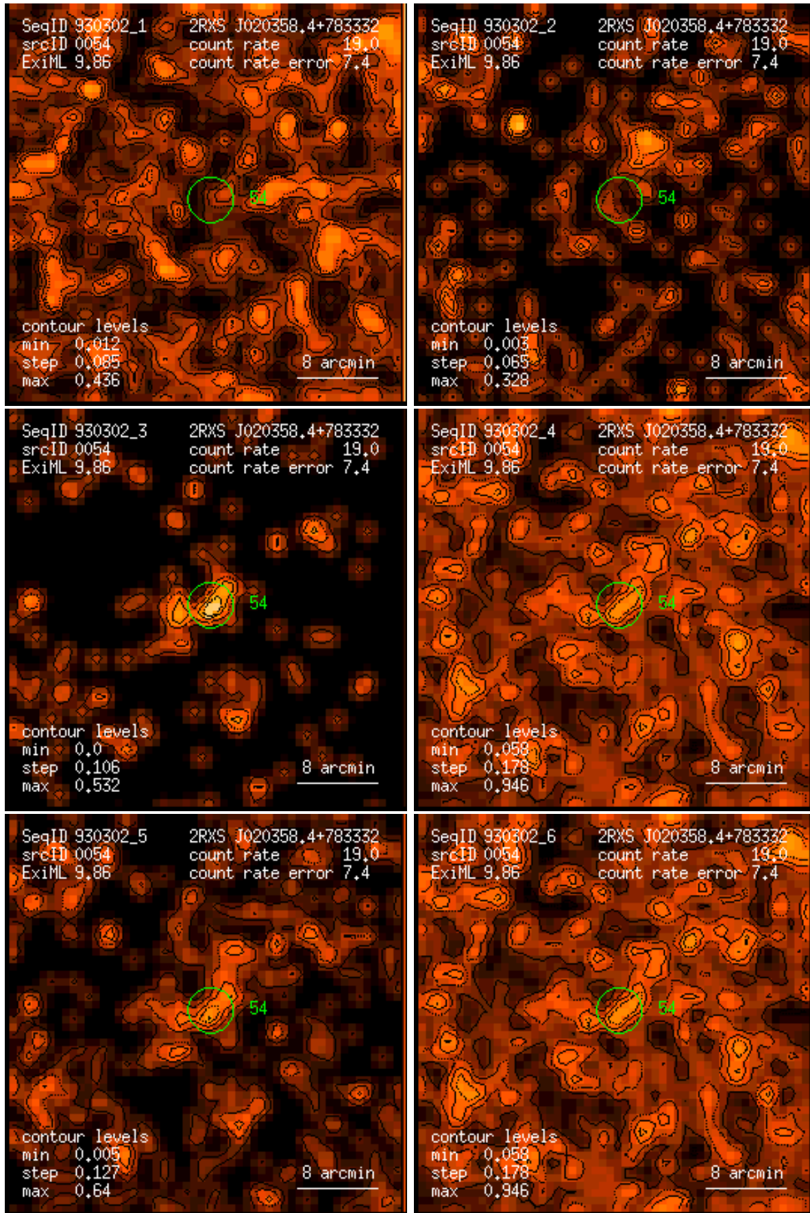
Figure 54: RASS 930302: detection 0054: band rate images, Gaussian filter: (1) PSPC channels 11 – 41, (2) 52 – 90, (3) 91 – 201, (4) 11 – 235, (5) 52 – 201, (6) 11 – 201. Broad band rates in counts/ks. Band rate contour levels in counts/ks/arcmin 2 .
