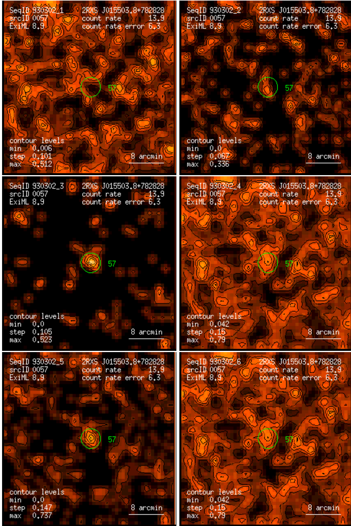
Figure 57: RASS 930302: detection 0057: band rate images, Gaussian filter: (1) PSPC channels 11 – 41, (2) 52 – 90, (3) 91 – 201, (4) 11 – 235, (5) 52 – 201, (6) 11 – 201. Broad band rates in counts/ks. Band rate contour levels in counts/ks/arcmin 2 .
