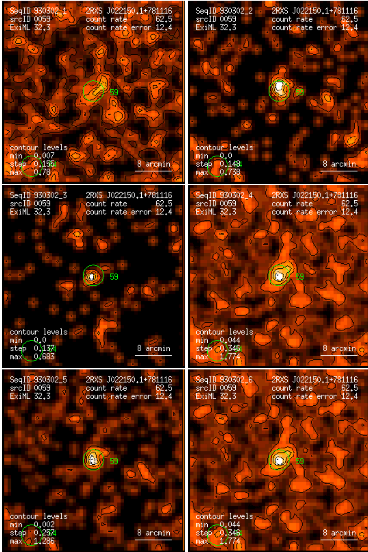
Figure 59: RASS 930302: detection 0059: band rate images, Gaussian filter: (1) PSPC channels 11 – 41, (2) 52 – 90, (3) 91 – 201, (4) 11 – 235, (5) 52 – 201, (6) 11 – 201. Broad band rates in counts/ks. Band rate contour levels in counts/ks/arcmin 2 .
