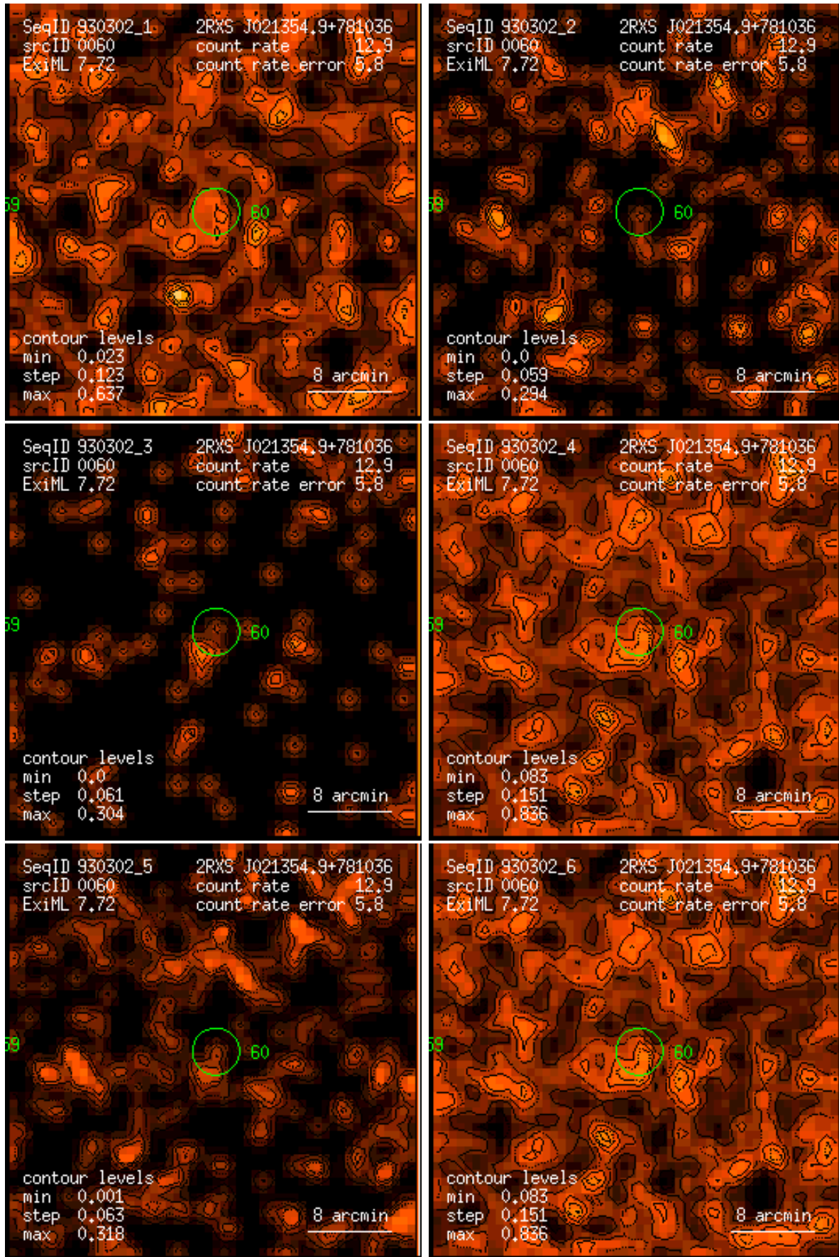
Figure 60: RASS 930302: detection 0060: band rate images, Gaussian filter: (1) PSPC channels 11 – 41, (2) 52 – 90, (3) 91 – 201, (4) 11 – 235, (5) 52 – 201, (6) 11 – 201. Broad band rates in counts/ks. Band rate contour levels in counts/ks/arcmin 2 .
