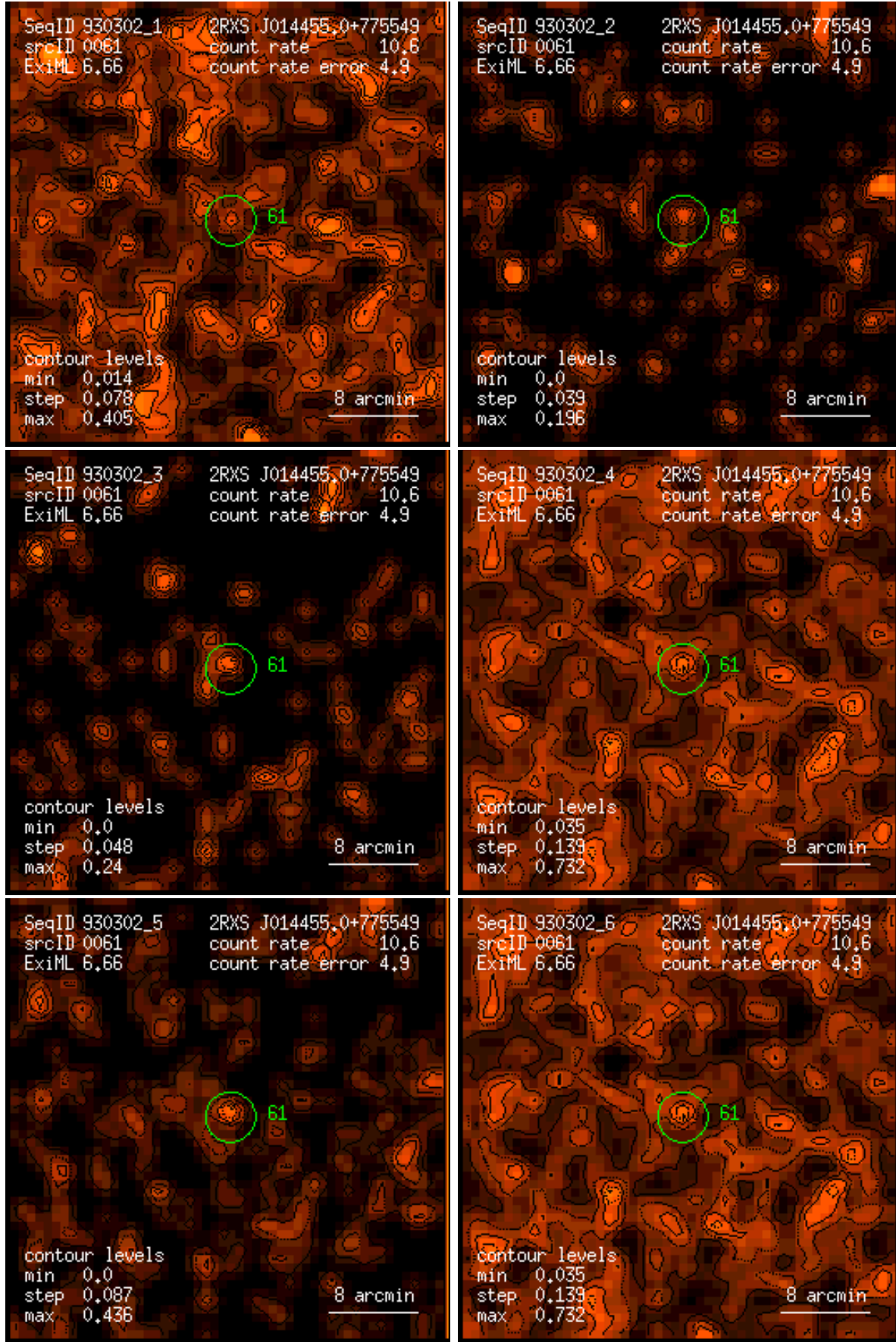
Figure 61: RASS 930302: detection 0061: band rate images, Gaussian filter: (1) PSPC channels 11 – 41, (2) 52 – 90, (3) 91 – 201, (4) 11 – 235, (5) 52 – 201, (6) 11 – 201. Broad band rates in counts/ks. Band rate contour levels in counts/ks/arcmin 2 .
