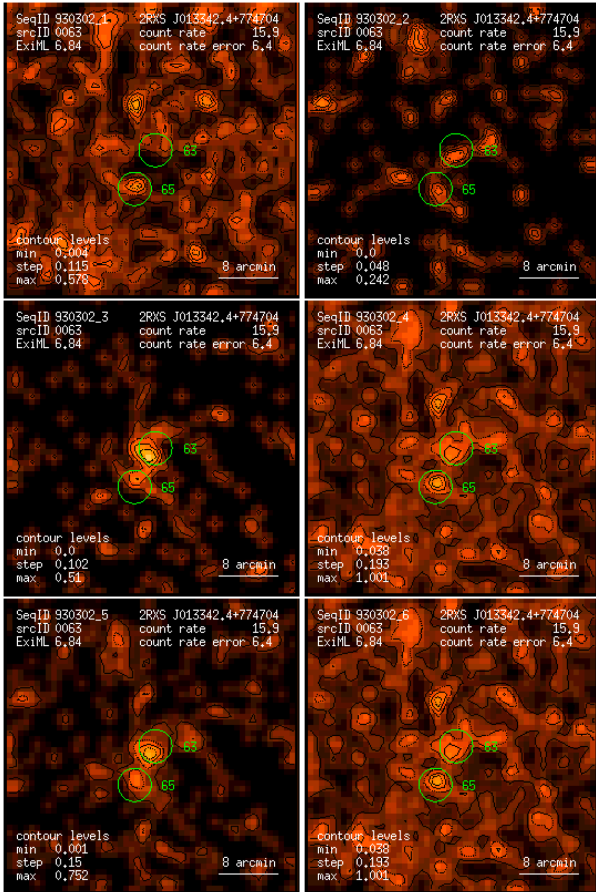
Figure 63: RASS 930302: detection 0063: band rate images, Gaussian filter: (1) PSPC channels 11 – 41, (2) 52 – 90, (3) 91 – 201, (4) 11 – 235, (5) 52 – 201, (6) 11 – 201. Broad band rates in counts/ks. Band rate contour levels in counts/ks/arcmin 2 .
