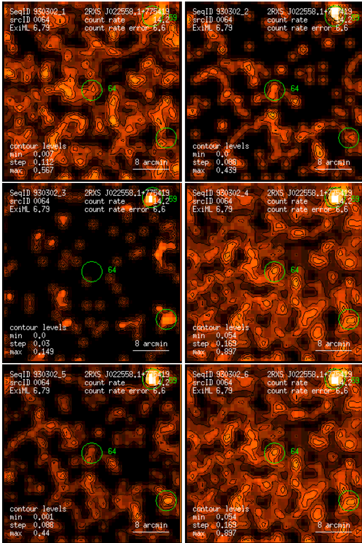
Figure 64: RASS 930302: detection 0064: band rate images, Gaussian filter: (1) PSPC channels 11 – 41, (2) 52 – 90, (3) 91 – 201, (4) 11 – 235, (5) 52 – 201, (6) 11 – 201. Broad band rates in counts/ks. Band rate contour levels in counts/ks/arcmin 2 .
