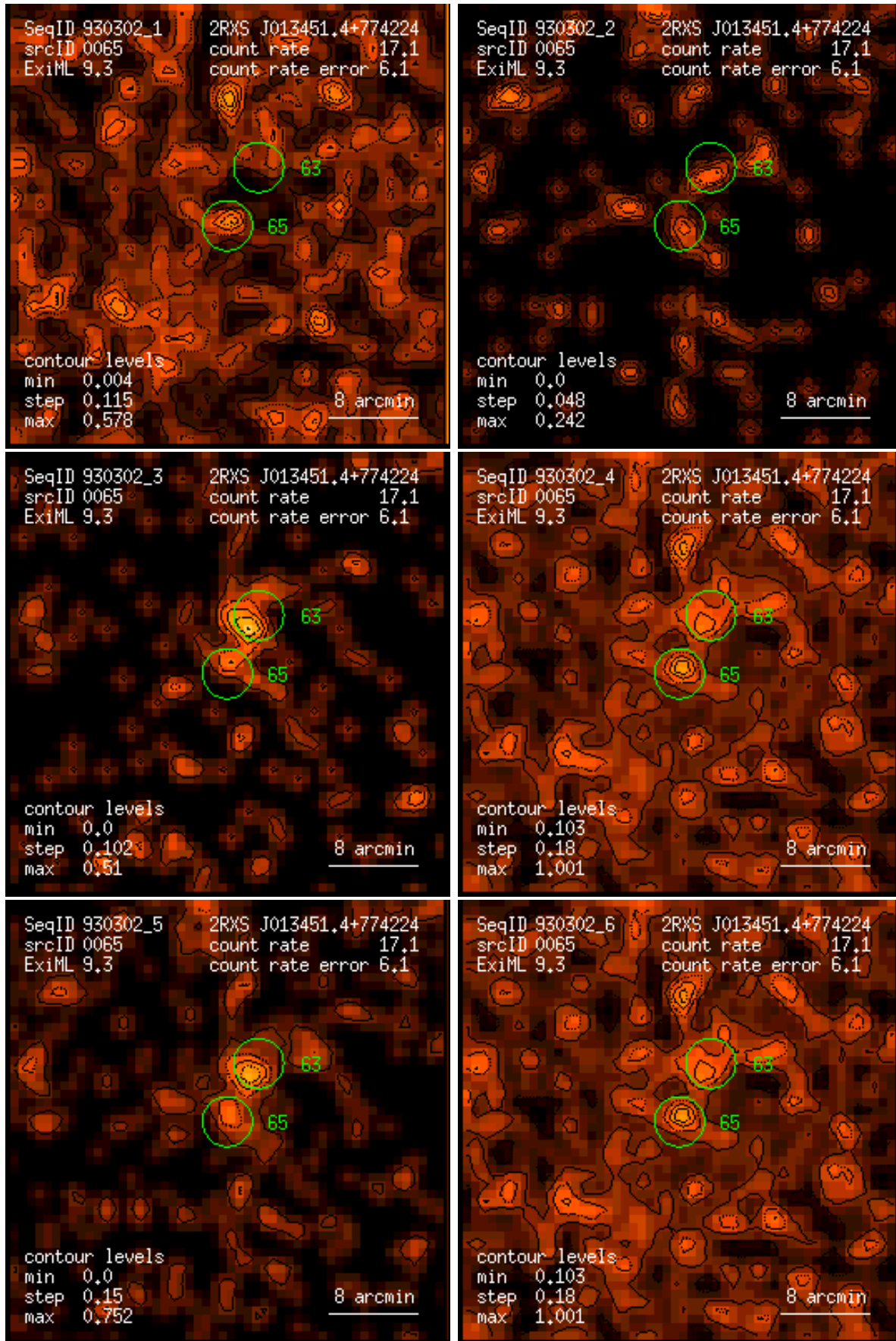
Figure 65: RASS 930302: detection 0065: band rate images, Gaussian filter: (1) PSPC channels 11 – 41, (2) 52 – 90, (3) 91 – 201, (4) 11 – 235, (5) 52 – 201, (6) 11 – 201. Broad band rates in counts/ks. Band rate contour levels in counts/ks/arcmin 2 .
