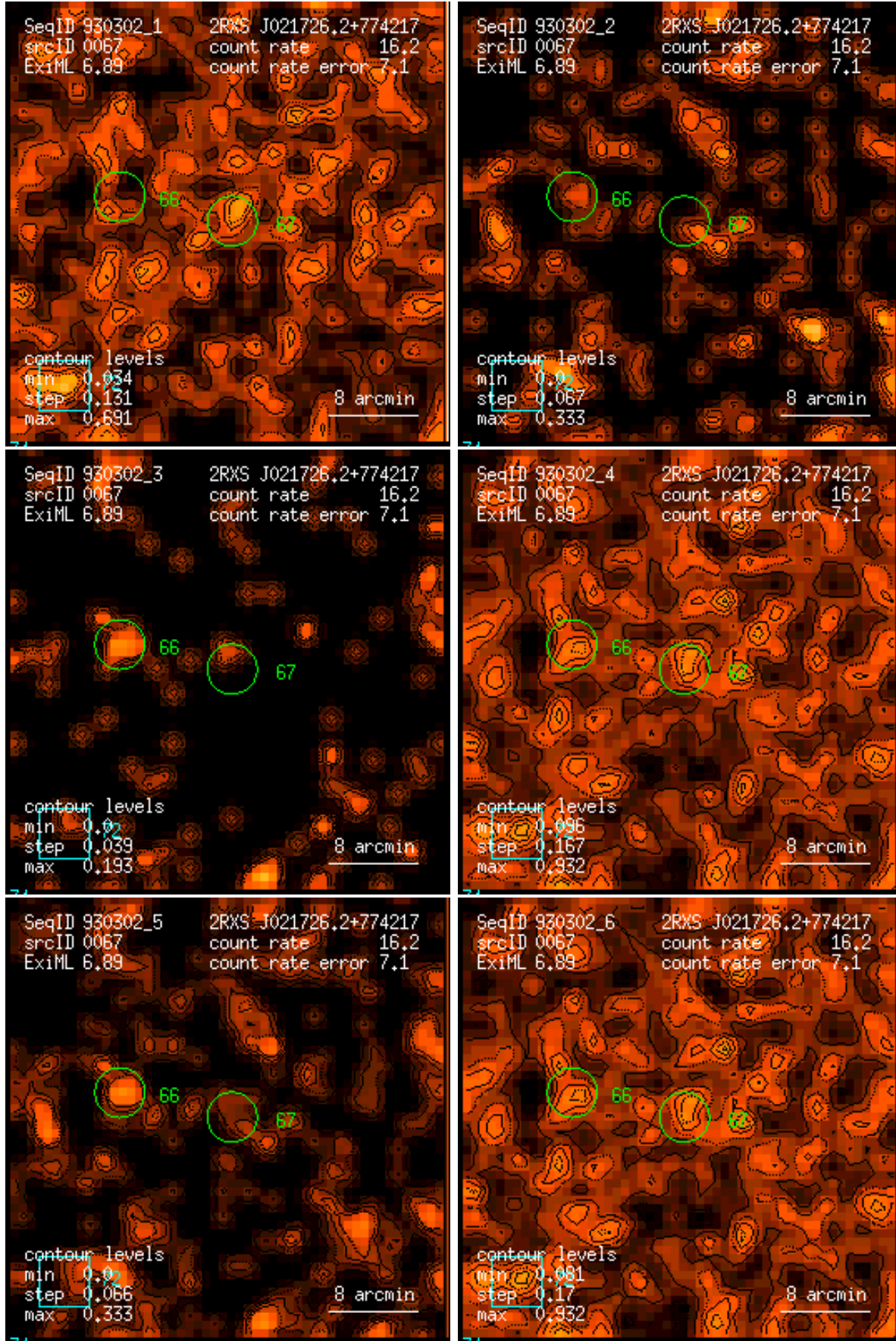
Figure 67: RASS 930302: detection 0067: band rate images, Gaussian filter: (1) PSPC channels 11 – 41, (2) 52 – 90, (3) 91 – 201, (4) 11 – 235, (5) 52 – 201, (6) 11 – 201. Broad band rates in counts/ks. Band rate contour levels in counts/ks/arcmin 2 .
