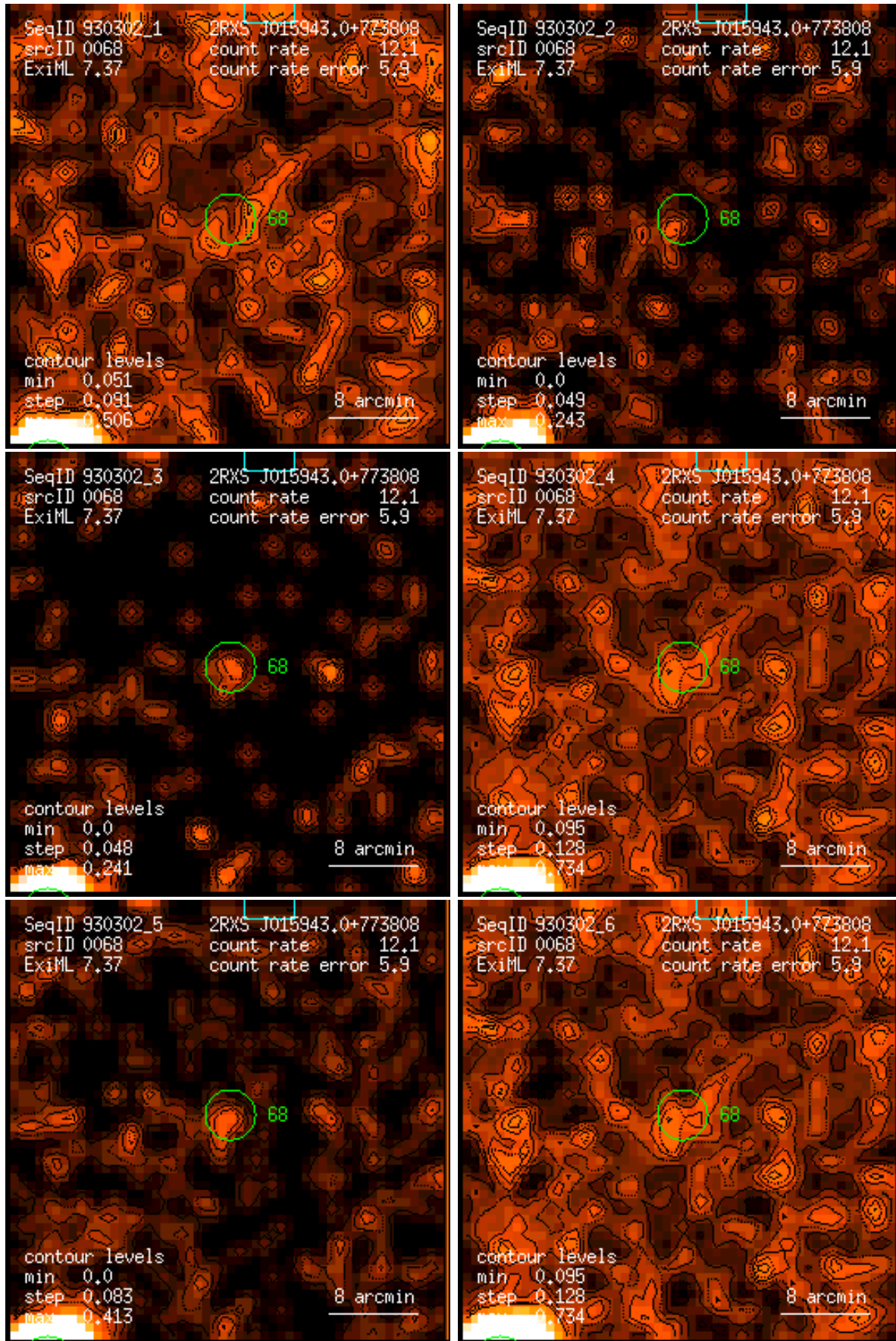
Figure 68: RASS 930302: detection 0068: band rate images, Gaussian filter: (1) PSPC channels 11 – 41, (2) 52 – 90, (3) 91 – 201, (4) 11 – 235, (5) 52 – 201, (6) 11 – 201. Broad band rates in counts/ks. Band rate contour levels in counts/ks/arcmin 2 .
