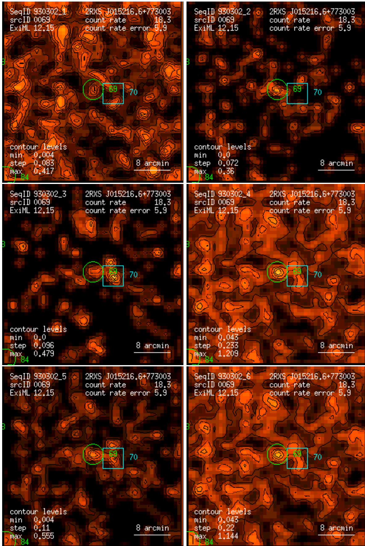
Figure 69: RASS 930302: detection 0069: band rate images, Gaussian filter: (1) PSPC channels 11 – 41, (2) 52 – 90, (3) 91 – 201, (4) 11 – 235, (5) 52 – 201, (6) 11 – 201. Broad band rates in counts/ks. Band rate contour levels in counts/ks/arcmin 2 .
