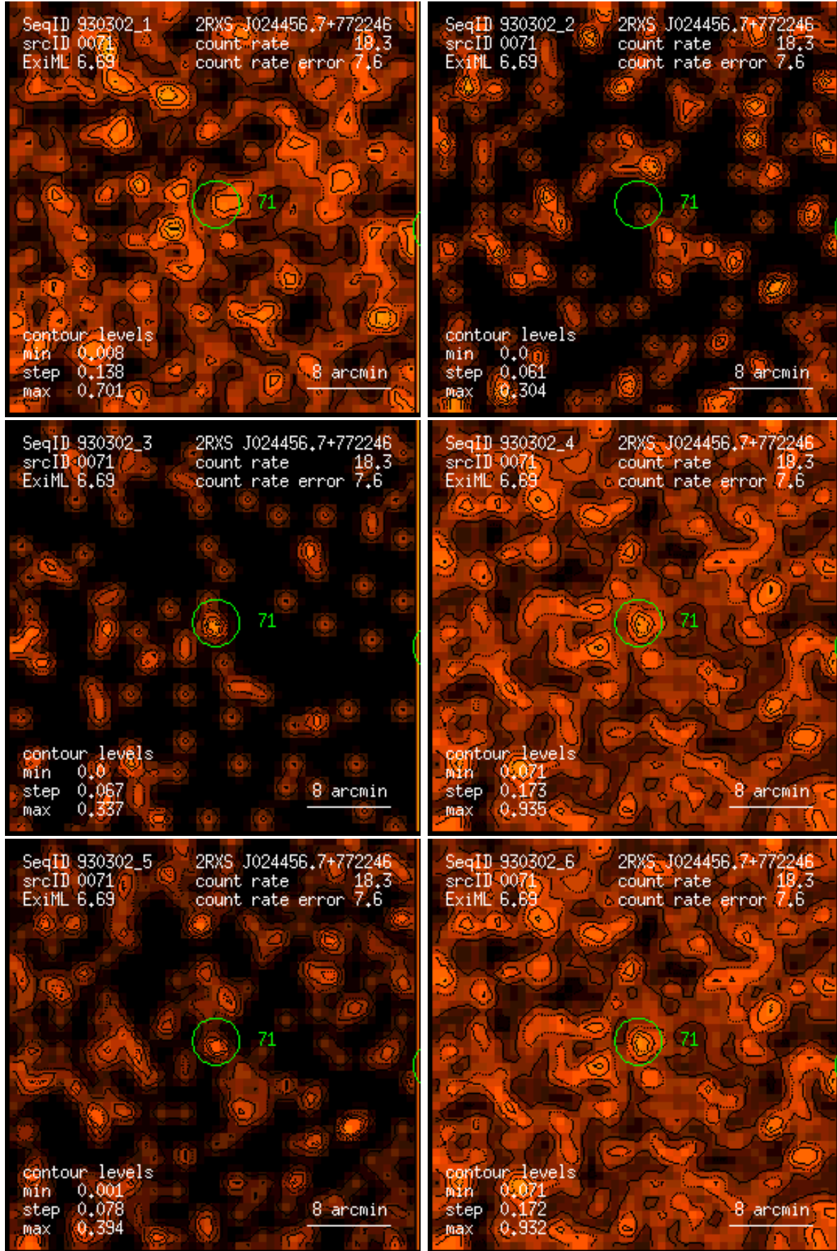
Figure 71: RASS 930302: detection 0071: band rate images, Gaussian filter: (1) PSPC channels 11 – 41, (2) 52 – 90, (3) 91 – 201, (4) 11 – 235, (5) 52 – 201, (6) 11 – 201. Broad band rates in counts/ks. Band rate contour levels in counts/ks/arcmin 2 .
