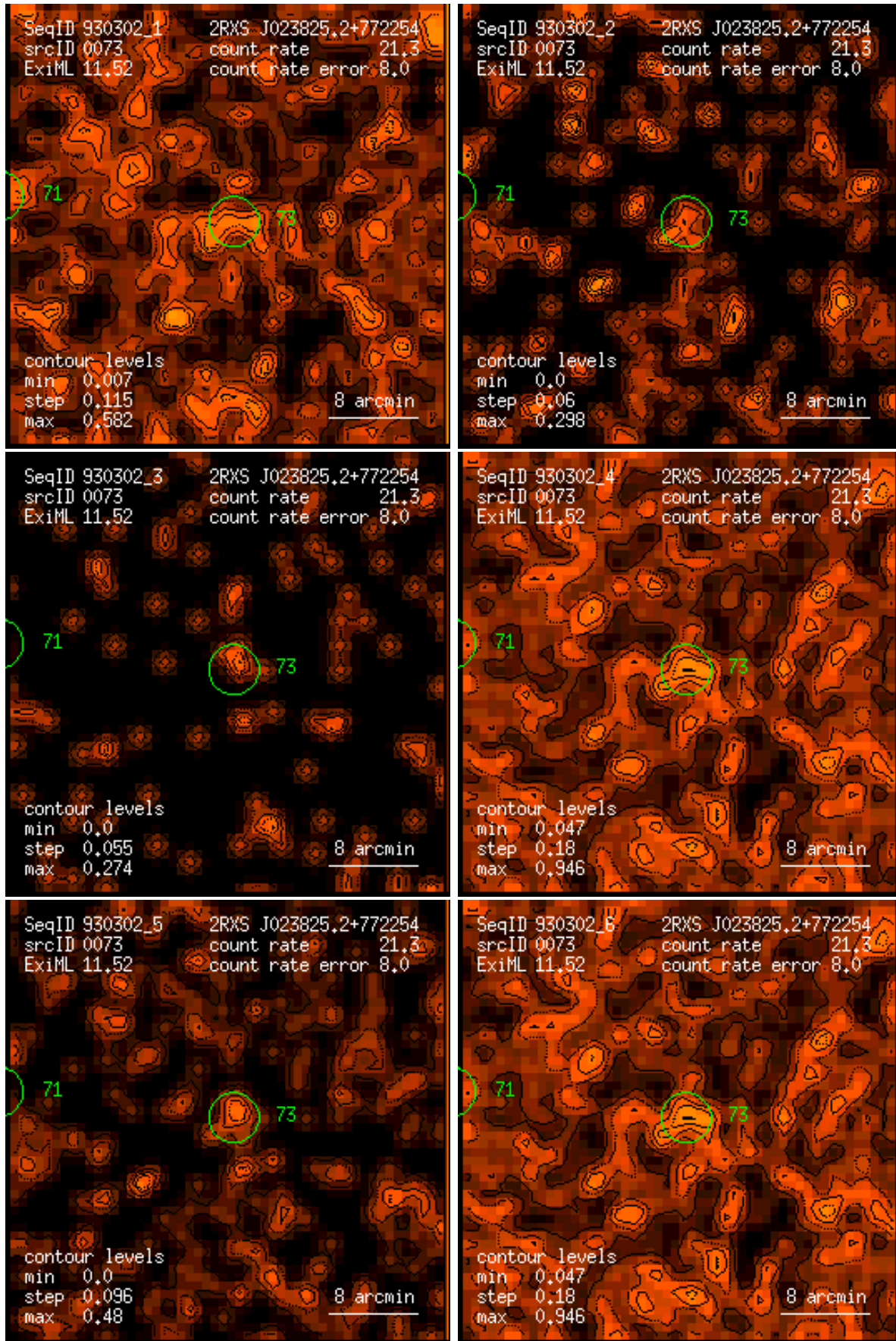
Figure 73: RASS 930302: detection 0073: band rate images, Gaussian filter: (1) PSPC channels 11 – 41, (2) 52 – 90, (3) 91 – 201, (4) 11 – 235, (5) 52 – 201, (6) 11 – 201. Broad band rates in counts/ks. Band rate contour levels in counts/ks/arcmin 2 .
