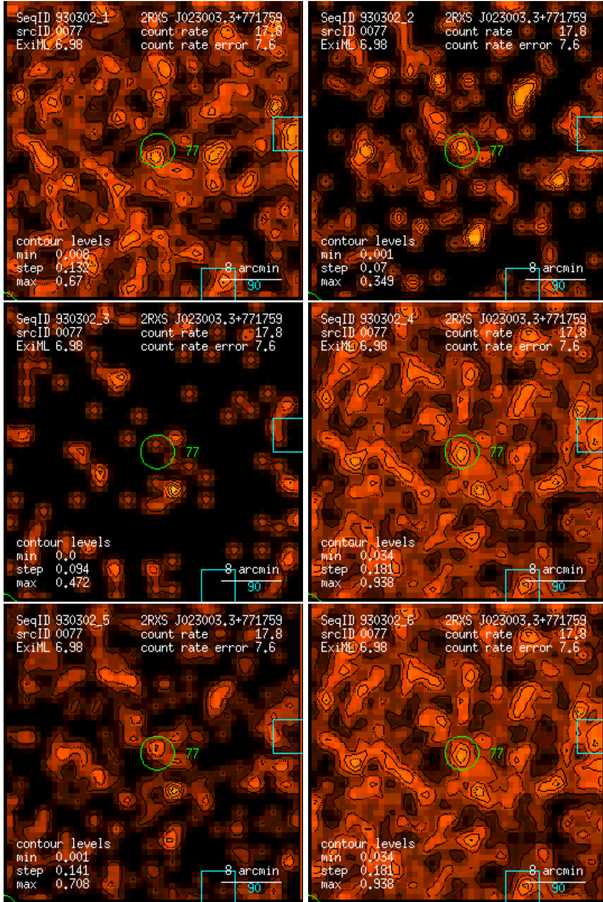
Figure 77: RASS 930302: detection 0077: band rate images, Gaussian filter: (1) PSPC channels 11 – 41, (2) 52 – 90, (3) 91 – 201, (4) 11 – 235, (5) 52 – 201, (6) 11 – 201. Broad band rates in counts/ks. Band rate contour levels in counts/ks/arcmin 2 .
