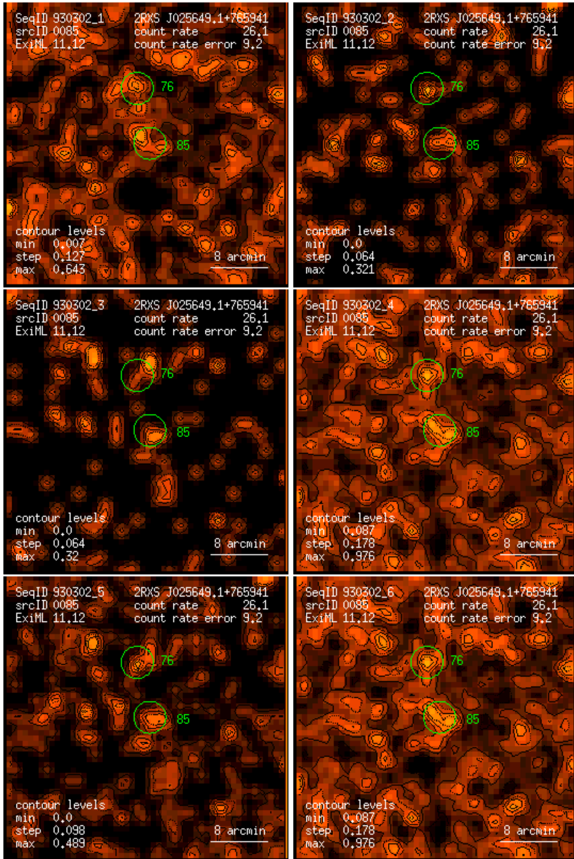
Figure 85: RASS 930302: detection 0085: band rate images, Gaussian filter: (1) PSPC channels 11 – 41, (2) 52 – 90, (3) 91 – 201, (4) 11 – 235, (5) 52 – 201, (6) 11 – 201. Broad band rates in counts/ks. Band rate contour levels in counts/ks/arcmin 2 .
