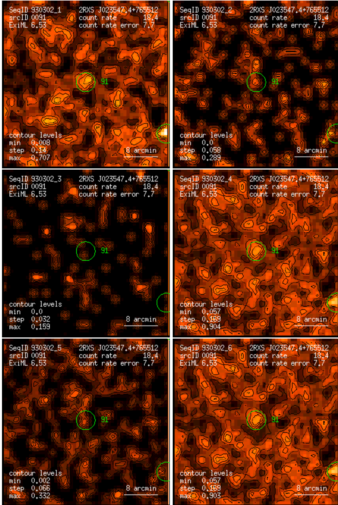
Figure 91: RASS 930302: detection 0091: band rate images, Gaussian filter: (1) PSPC channels 11 – 41, (2) 52 – 90, (3) 91 – 201, (4) 11 – 235, (5) 52 – 201, (6) 11 – 201. Broad band rates in counts/ks. Band rate contour levels in counts/ks/arcmin 2 .
