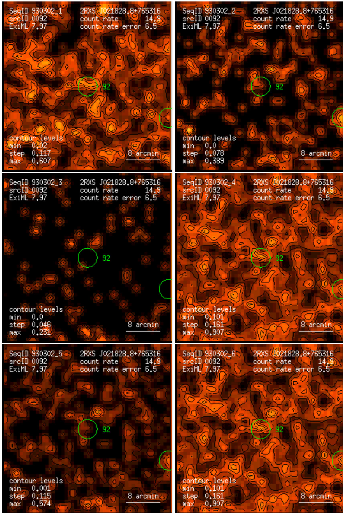
Figure 92: RASS 930302: detection 0092: band rate images, Gaussian filter: (1) PSPC channels 11 – 41, (2) 52 – 90, (3) 91 – 201, (4) 11 – 235, (5) 52 – 201, (6) 11 – 201. Broad band rates in counts/ks. Band rate contour levels in counts/ks/arcmin 2 .
