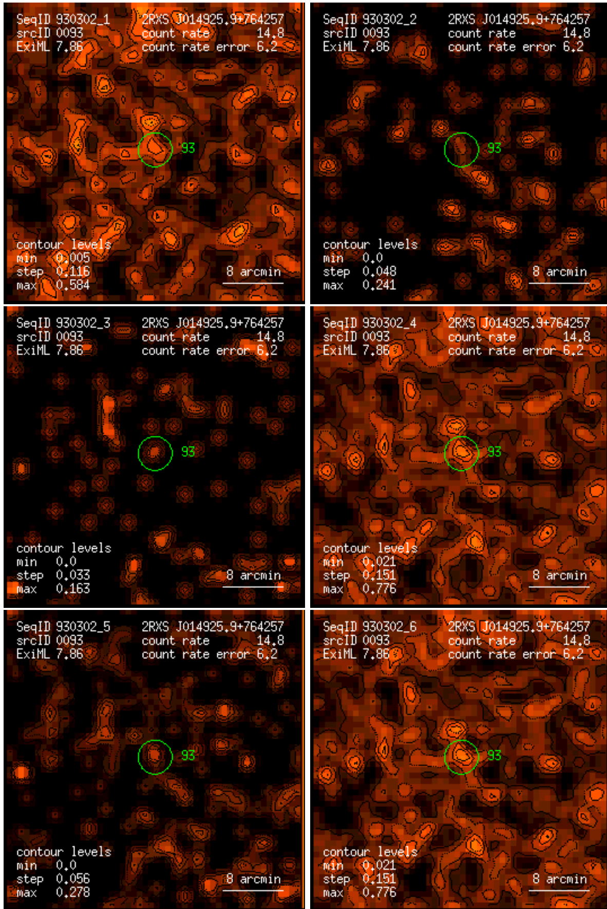
Figure 93: RASS 930302: detection 0093: band rate images, Gaussian filter: (1) PSPC channels 11 – 41, (2) 52 – 90, (3) 91 – 201, (4) 11 – 235, (5) 52 – 201, (6) 11 – 201. Broad band rates in counts/ks. Band rate contour levels in counts/ks/arcmin 2 .
