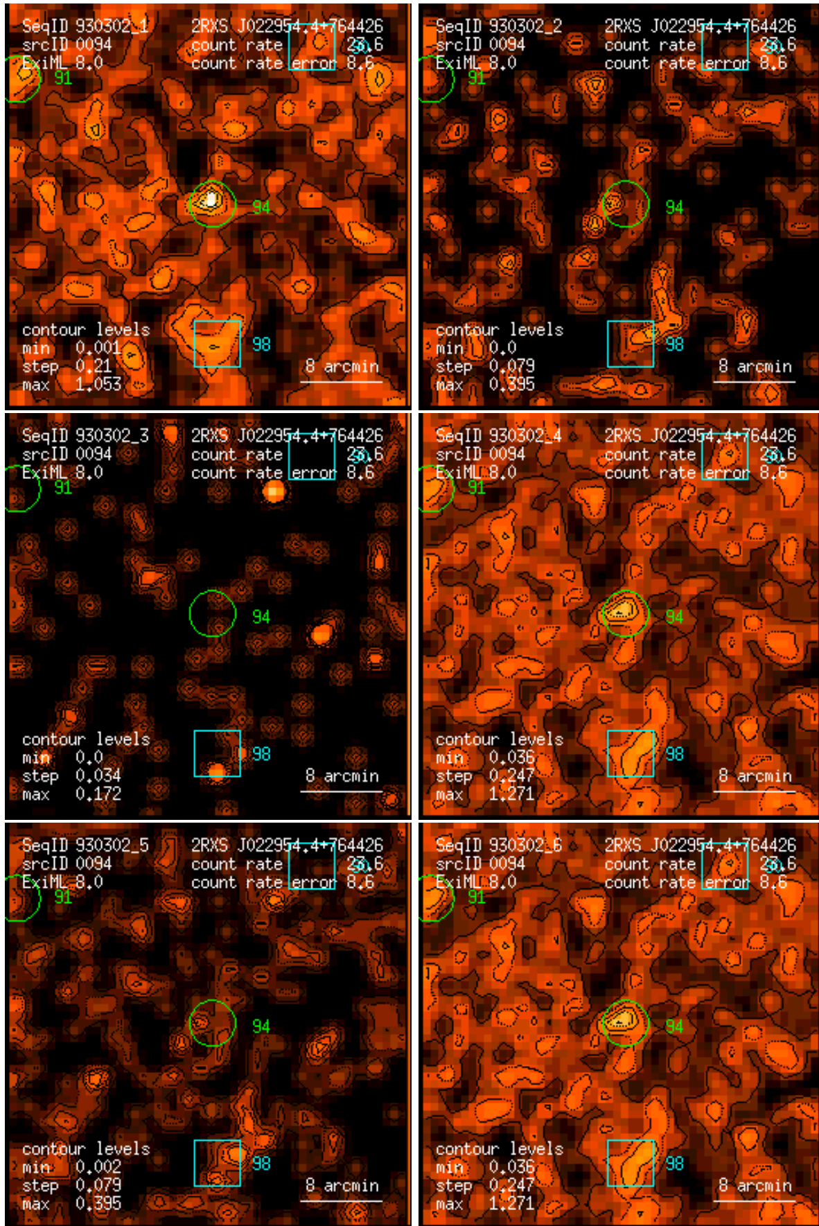
Figure 94: RASS 930302: detection 0094: band rate images, Gaussian filter: (1) PSPC channels 11 – 41, (2) 52 – 90, (3) 91 – 201, (4) 11 – 235, (5) 52 – 201, (6) 11 – 201. Broad band rates in counts/ks. Band rate contour levels in counts/ks/arcmin 2 .
