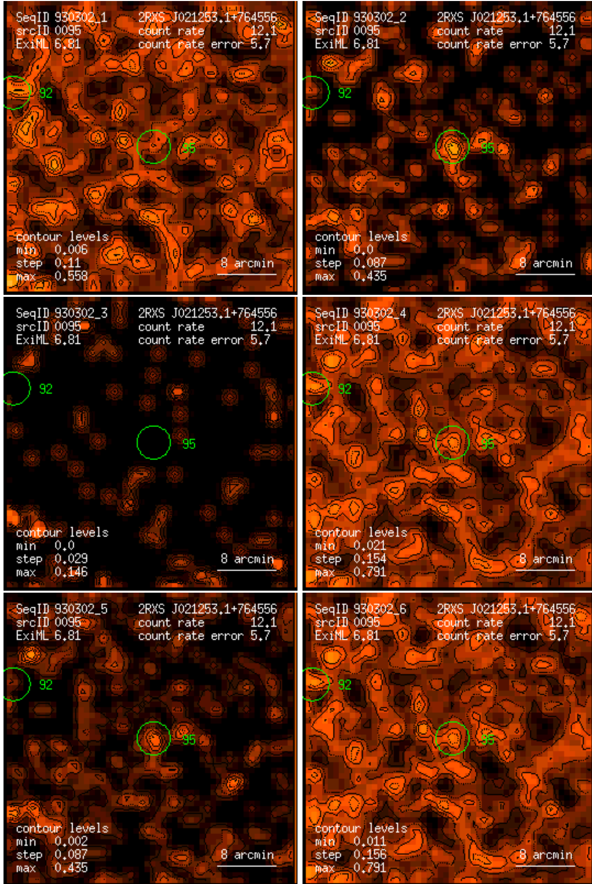
Figure 95: RASS 930302: detection 0095: band rate images, Gaussian filter: (1) PSPC channels 11 – 41, (2) 52 – 90, (3) 91 – 201, (4) 11 – 235, (5) 52 – 201, (6) 11 – 201. Broad band rates in counts/ks. Band rate contour levels in counts/ks/arcmin 2 .
