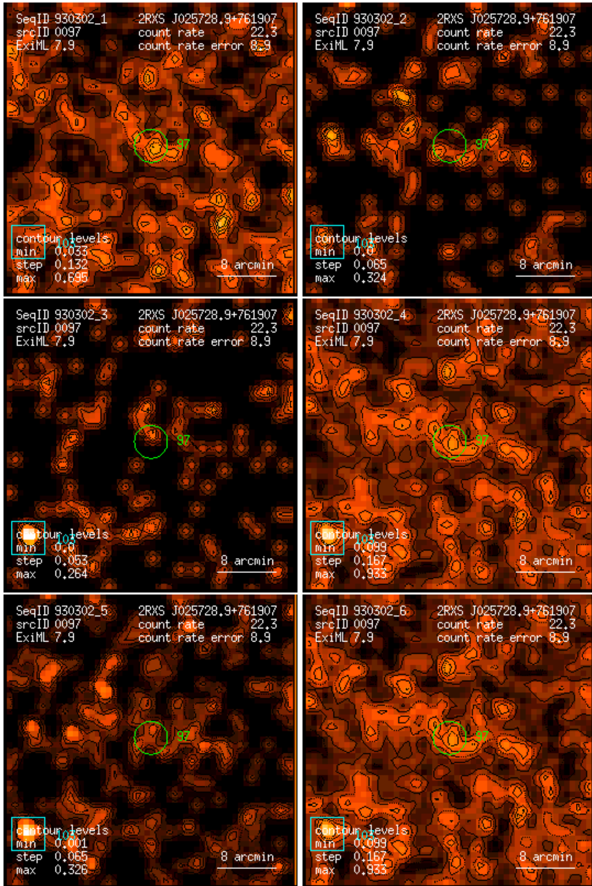
Figure 97: RASS 930302: detection 0097: band rate images, Gaussian filter: (1) PSPC channels 11 – 41, (2) 52 – 90, (3) 91 – 201, (4) 11 – 235, (5) 52 – 201, (6) 11 – 201. Broad band rates in counts/ks. Band rate contour levels in counts/ks/arcmin 2 .
