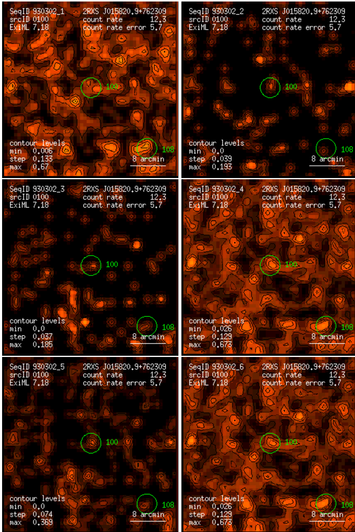
Figure 100: RASS 930302: detection 0100: band rate images, Gaussian filter: (1) PSPC channels 11 – 41, (2) 52 – 90, (3) 91 – 201, (4) 11 – 235, (5) 52 – 201, (6) 11 – 201. Broad band rates in counts/ks. Band rate contour levels in counts/ks/arcmin 2 .
