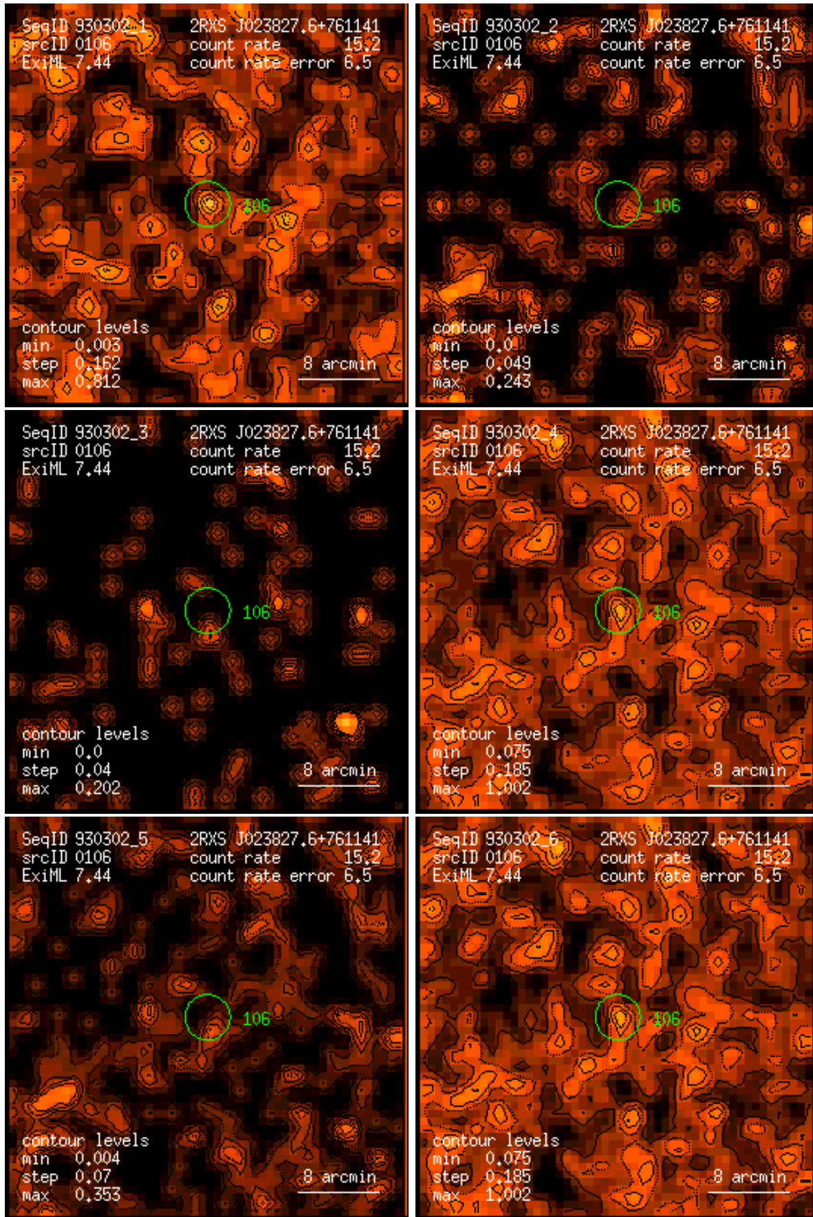
Figure 106: RASS 930302: detection 0106: band rate images, Gaussian filter: (1) PSPC channels 11 – 41, (2) 52 – 90, (3) 91 – 201, (4) 11 – 235, (5) 52 – 201, (6) 11 – 201. Broad band rates in counts/ks. Band rate contour levels in counts/ks/arcmin 2 .
