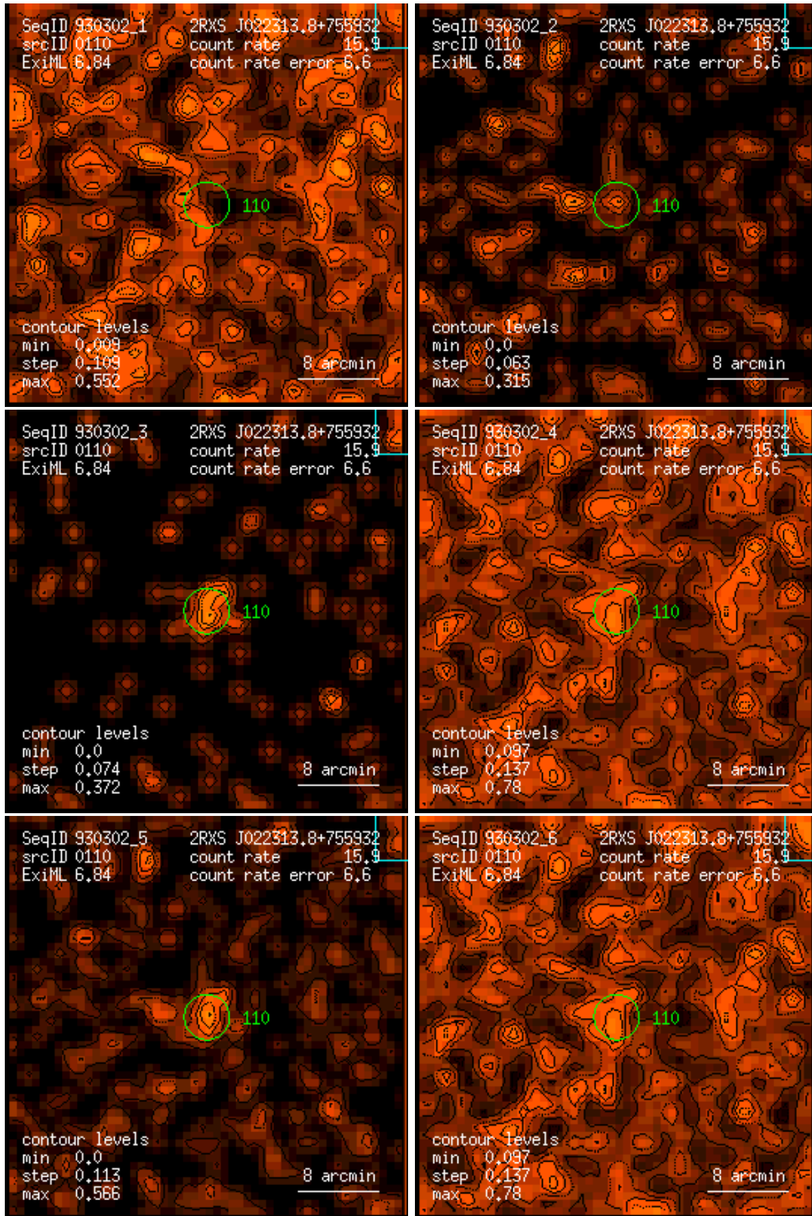
Figure 110: RASS 930302: detection 0110: band rate images, Gaussian filter: (1) PSPC channels 11 – 41, (2) 52 – 90, (3) 91 – 201, (4) 11 – 235, (5) 52 – 201, (6) 11 – 201. Broad band rates in counts/ks. Band rate contour levels in counts/ks/arcmin 2 .
