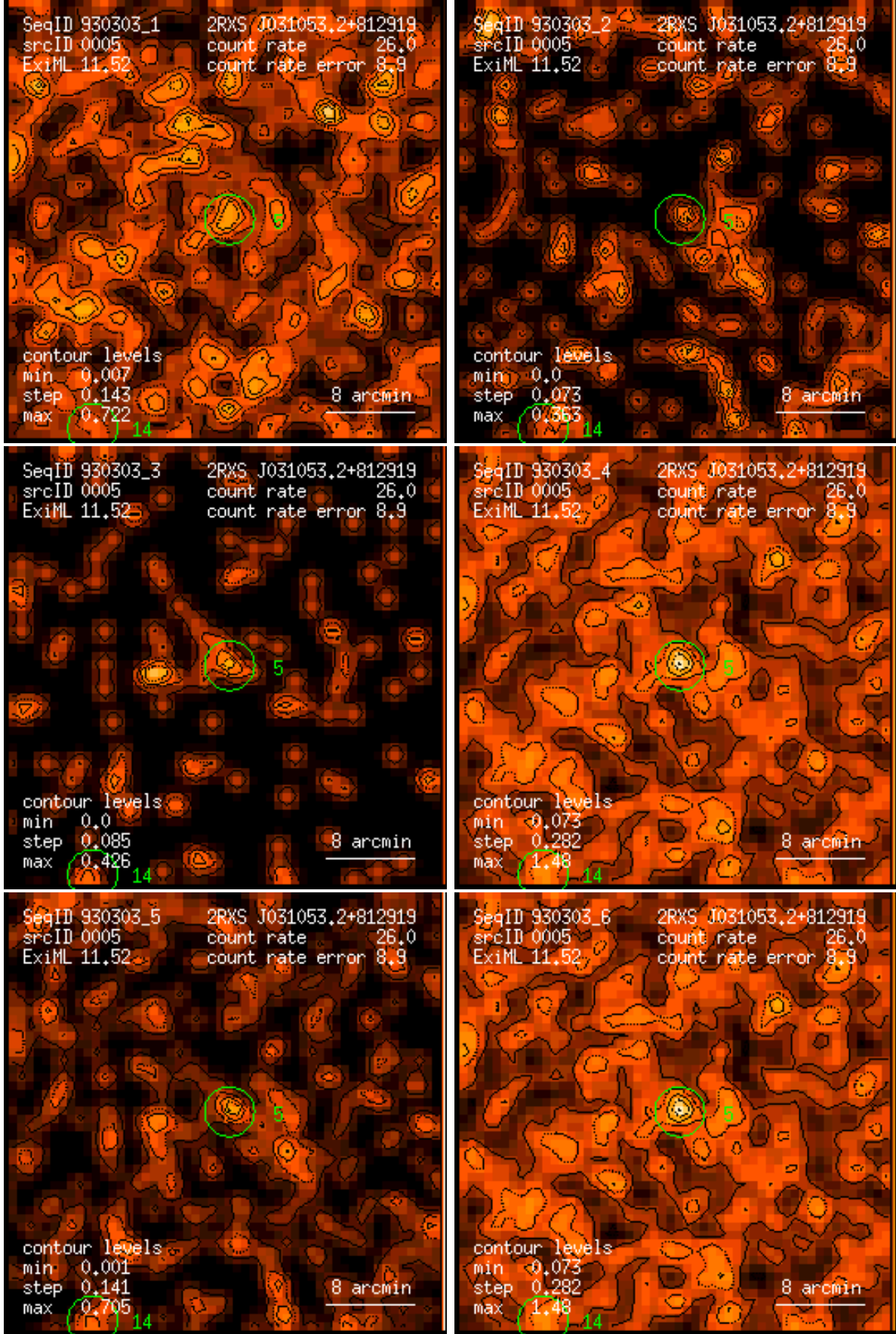
Figure 5: RASS 930303: detection 0005: band rate images, Gaussian filter: (1) PSPC channels 11 – 41, (2) 52 – 90, (3) 91 – 201, (4) 11 – 235, (5) 52 – 201, (6) 11 – 201. Broad band rates in counts/ks. Band rate contour levels in counts/ks/arcmin 2 .
