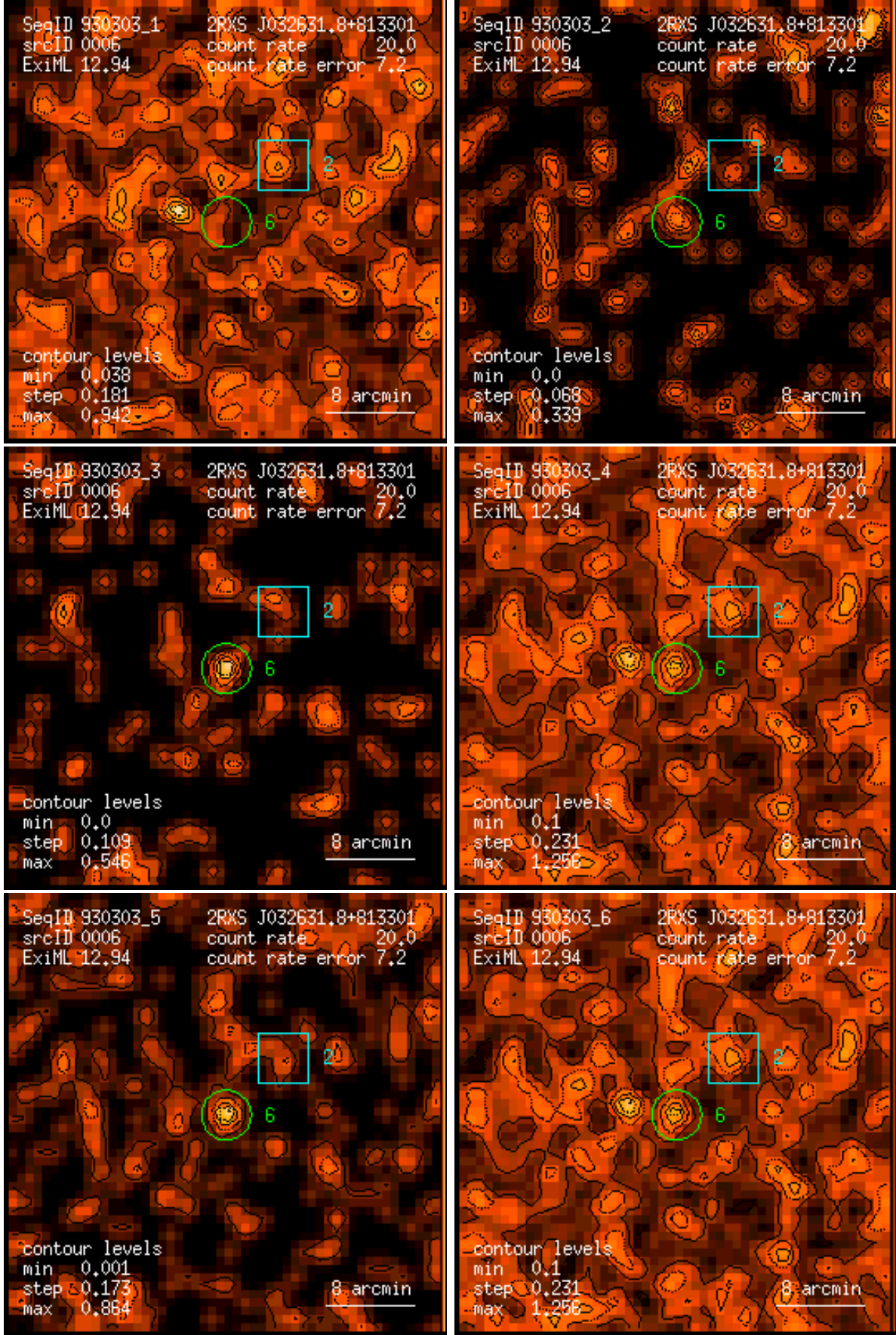
Figure 6: RASS 930303: detection 0006: band rate images, Gaussian filter: (1) PSPC channels 11 – 41, (2) 52 – 90, (3) 91 – 201, (4) 11 – 235, (5) 52 – 201, (6) 11 – 201. Broad band rates in counts/ks. Band rate contour levels in counts/ks/arcmin 2 .
