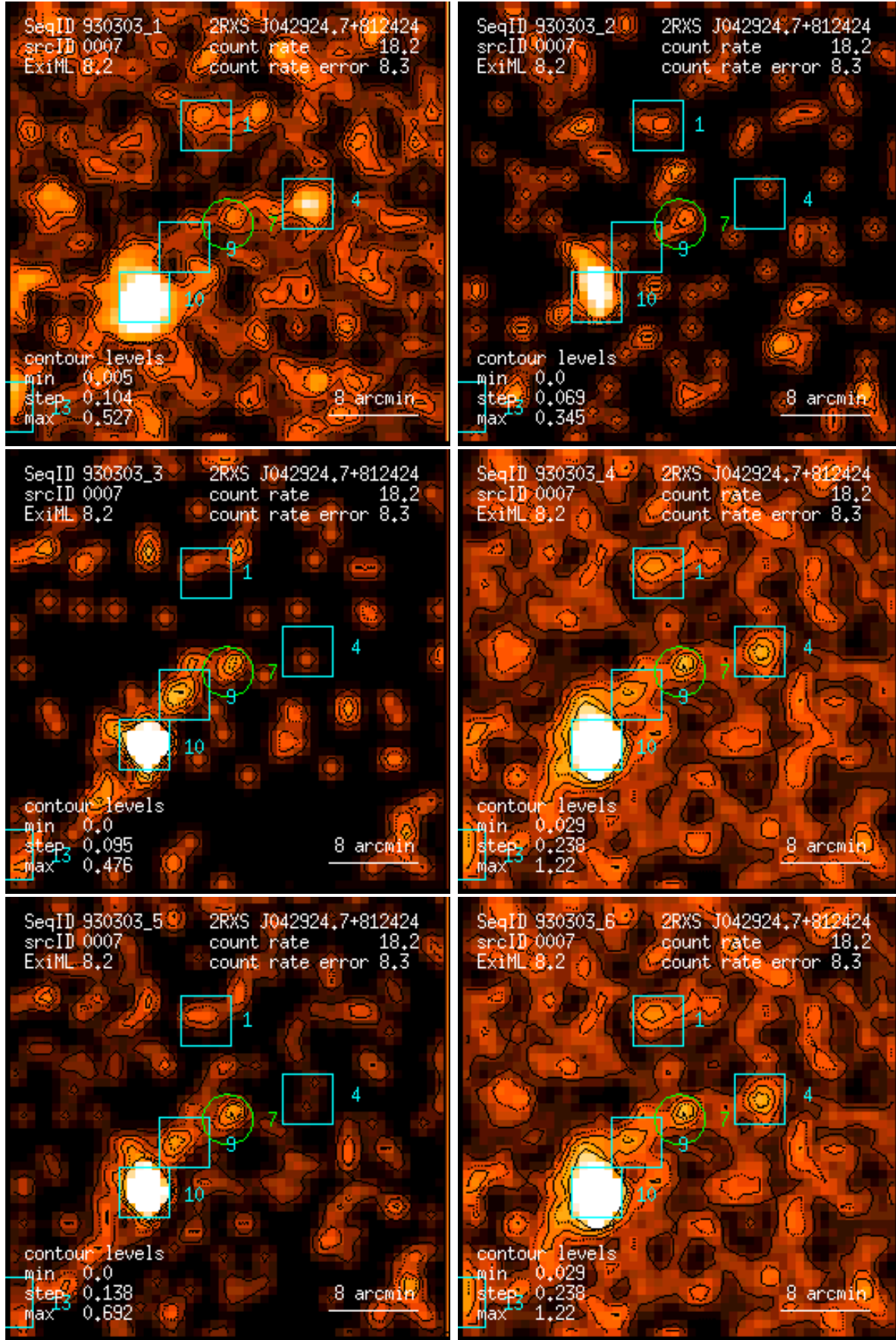
Figure 7: RASS 930303: detection 0007: band rate images, Gaussian filter: (1) PSPC channels 11 – 41, (2) 52 – 90, (3) 91 – 201, (4) 11 – 235, (5) 52 – 201, (6) 11 – 201. Broad band rates in counts/ks. Band rate contour levels in counts/ks/arcmin 2 .
