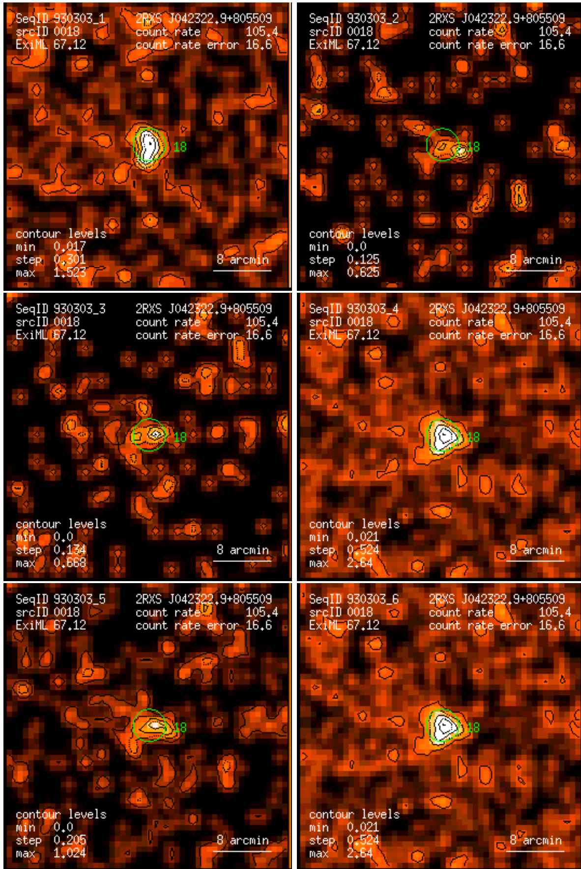
Figure 18: RASS 930303: detection 0018: band rate images, Gaussian filter: (1) PSPC channels 11 – 41, (2) 52 – 90, (3) 91 – 201, (4) 11 – 235, (5) 52 – 201, (6) 11 – 201. Broad band rates in counts/ks. Band rate contour levels in counts/ks/arcmin 2 .
