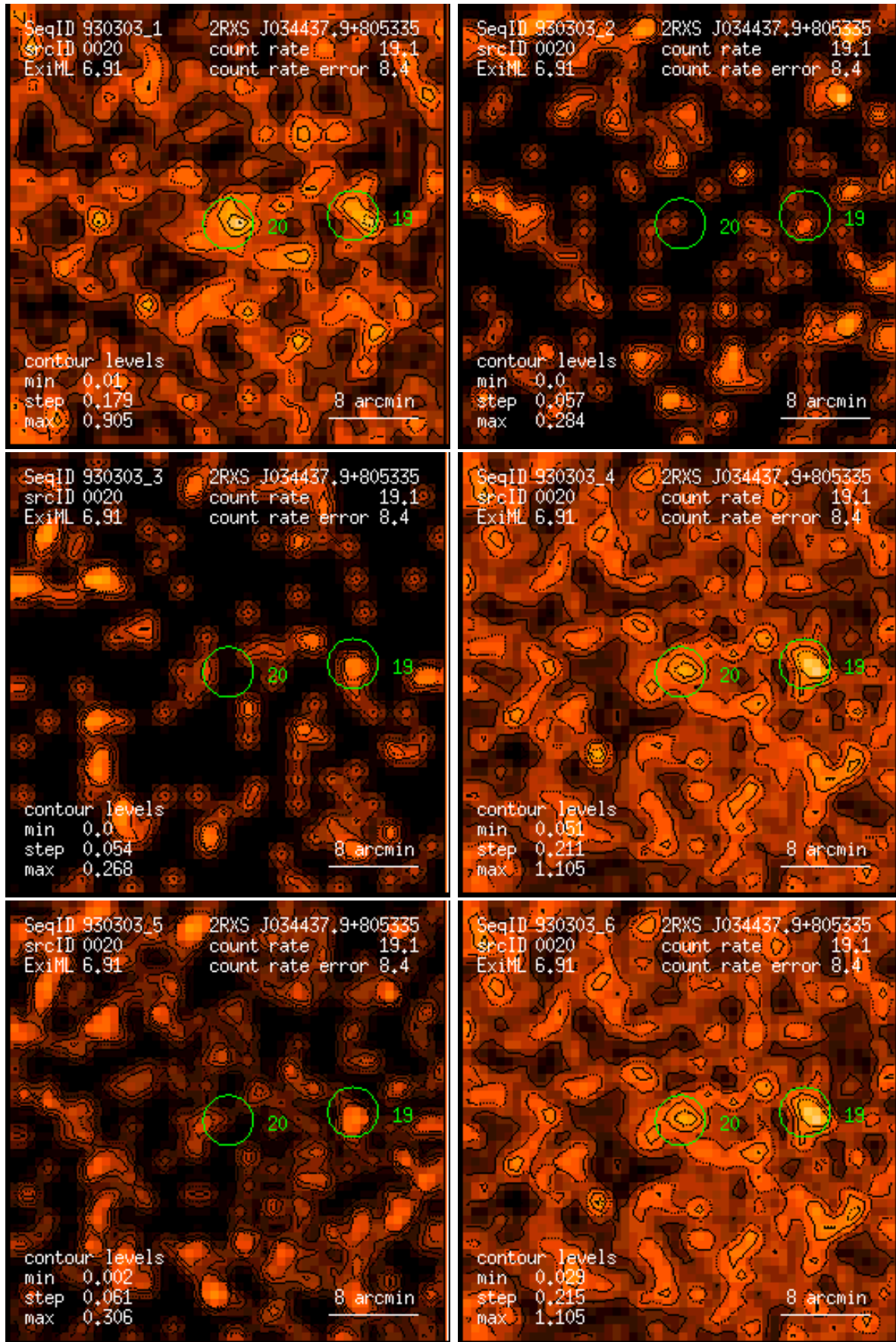
Figure 20: RASS 930303: detection 0020: band rate images, Gaussian filter: (1) PSPC channels 11 – 41, (2) 52 – 90, (3) 91 – 201, (4) 11 – 235, (5) 52 – 201, (6) 11 – 201. Broad band rates in counts/ks. Band rate contour levels in counts/ks/arcmin 2 .
