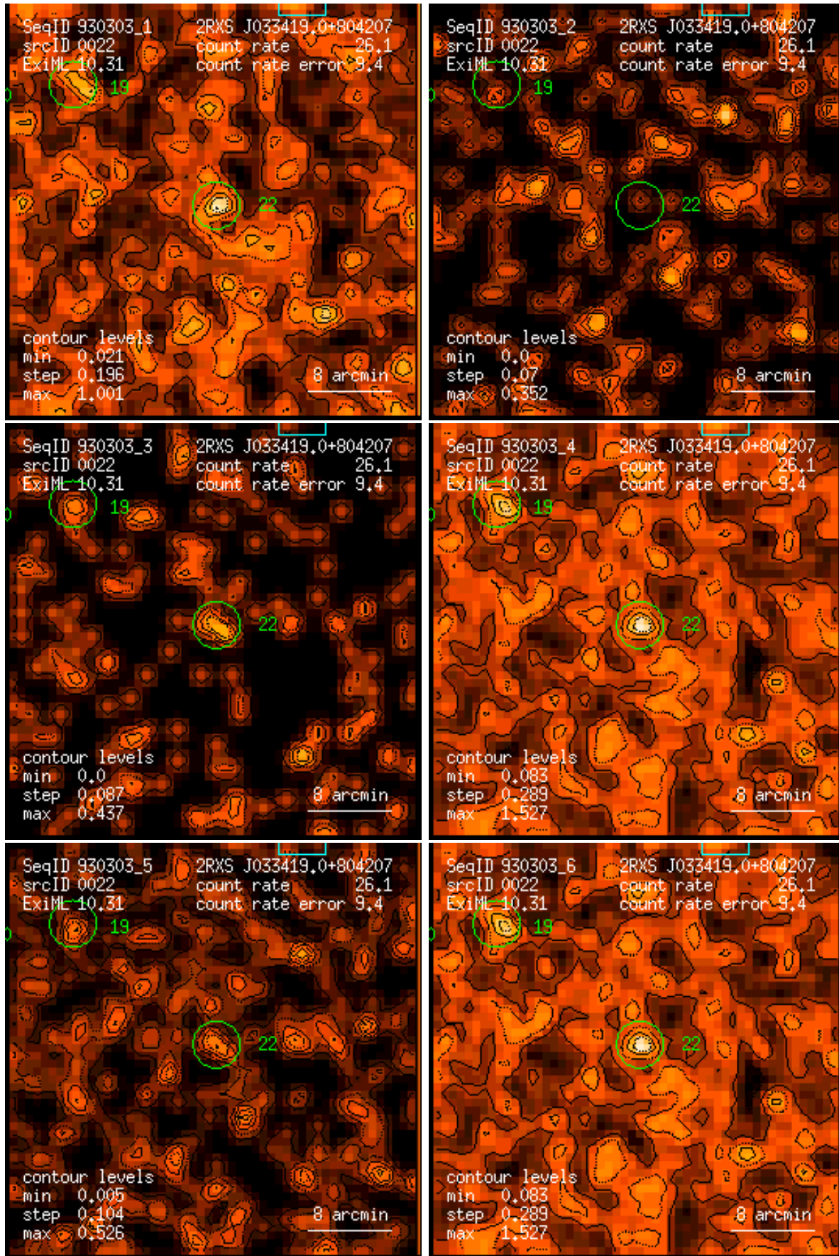
Figure 22: RASS 930303: detection 0022: band rate images, Gaussian filter: (1) PSPC channels 11 – 41, (2) 52 – 90, (3) 91 – 201, (4) 11 – 235, (5) 52 – 201, (6) 11 – 201. Broad band rates in counts/ks. Band rate contour levels in counts/ks/arcmin 2 .
