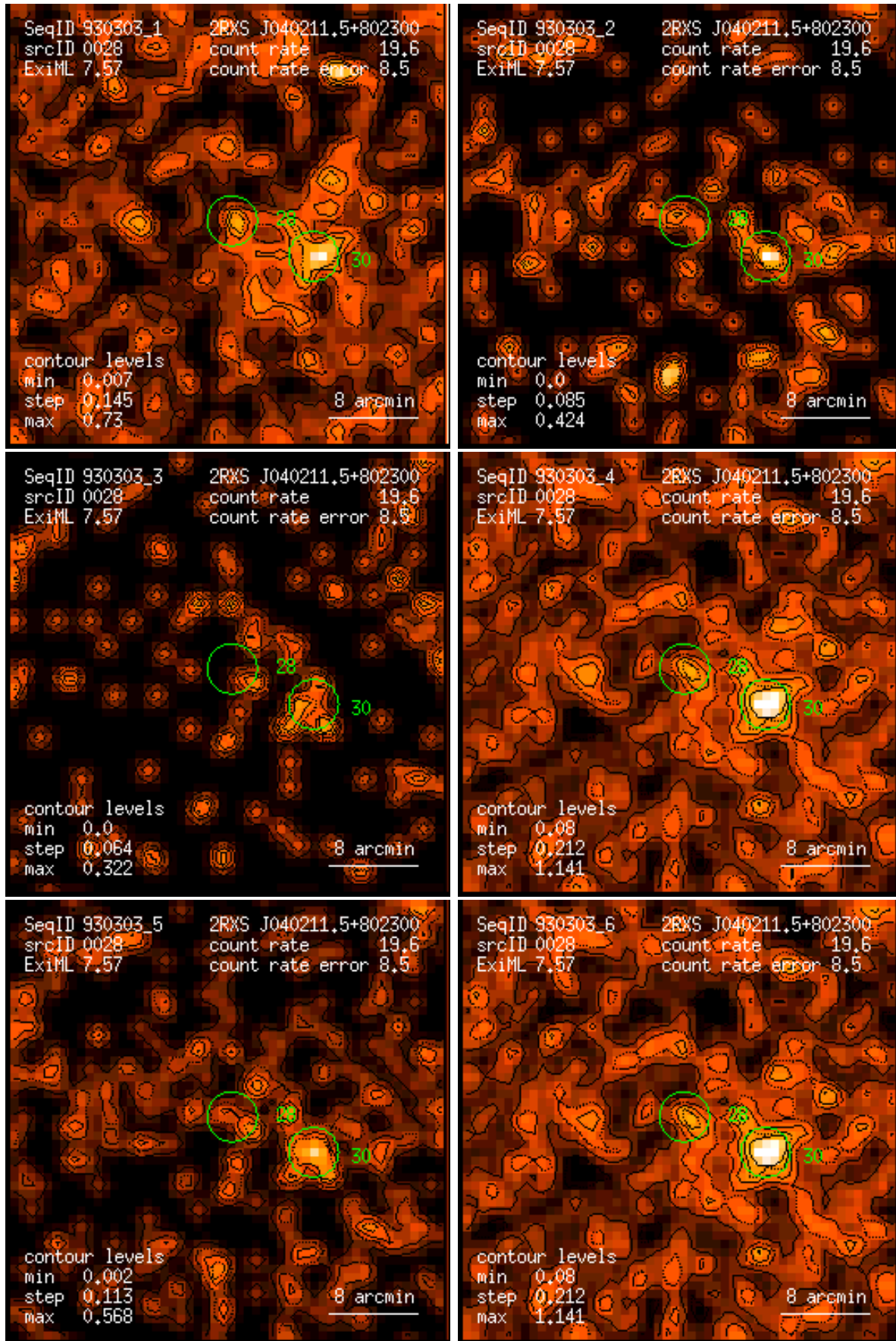
Figure 28: RASS 930303: detection 0028: band rate images, Gaussian filter: (1) PSPC channels 11 – 41, (2) 52 – 90, (3) 91 – 201, (4) 11 – 235, (5) 52 – 201, (6) 11 – 201. Broad band rates in counts/ks. Band rate contour levels in counts/ks/arcmin 2 .
