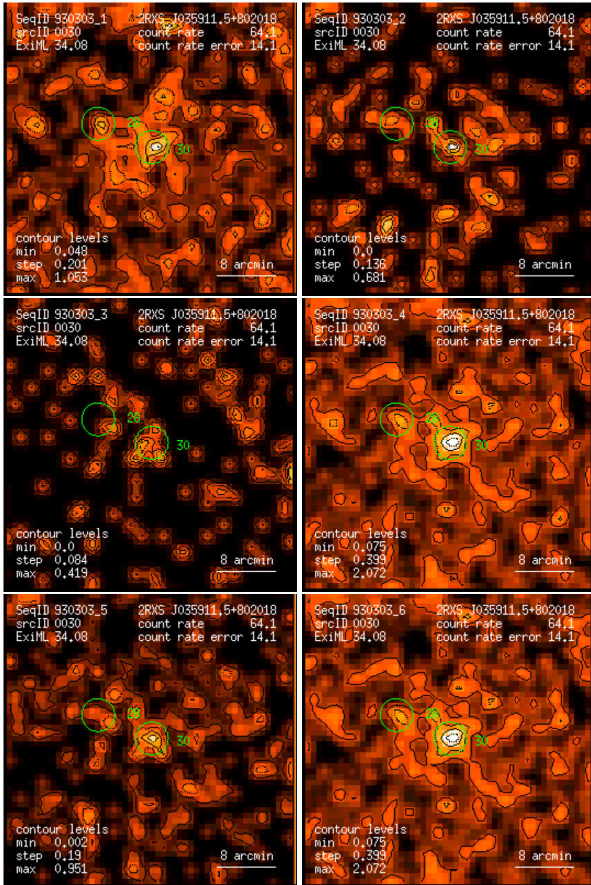
Figure 30: RASS 930303: detection 0030: band rate images, Gaussian filter: (1) PSPC channels 11 – 41, (2) 52 – 90, (3) 91 – 201, (4) 11 – 235, (5) 52 – 201, (6) 11 – 201. Broad band rates in counts/ks. Band rate contour levels in counts/ks/arcmin 2 .
