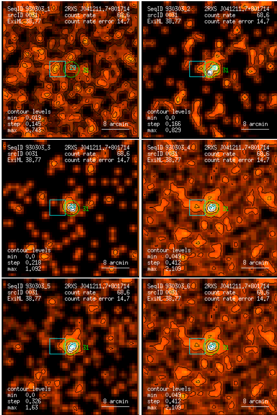
Figure 31: RASS 930303: detection 0031: band rate images, Gaussian filter: (1) PSPC channels 11 – 41, (2) 52 – 90, (3) 91 – 201, (4) 11 – 235, (5) 52 – 201, (6) 11 – 201. Broad band rates in counts/ks. Band rate contour levels in counts/ks/arcmin 2 .
