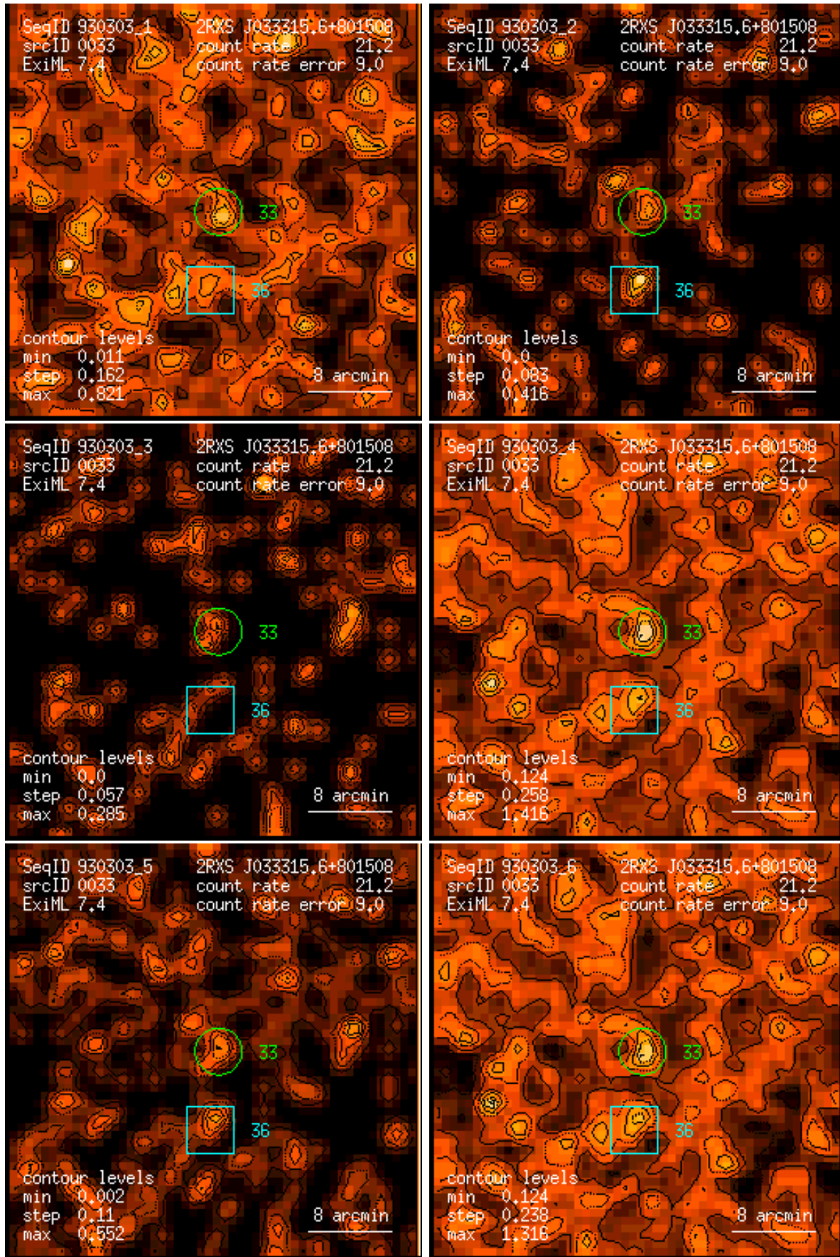
Figure 33: RASS 930303: detection 0033: band rate images, Gaussian filter: (1) PSPC channels 11 – 41, (2) 52 – 90, (3) 91 – 201, (4) 11 – 235, (5) 52 – 201, (6) 11 – 201. Broad band rates in counts/ks. Band rate contour levels in counts/ks/arcmin 2 .
