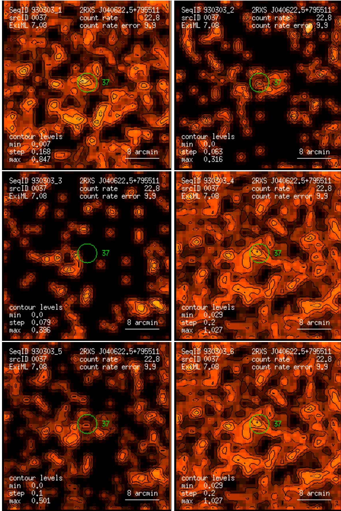
Figure 37: RASS 930303: detection 0037: band rate images, Gaussian filter: (1) PSPC channels 11 – 41, (2) 52 – 90, (3) 91 – 201, (4) 11 – 235, (5) 52 – 201, (6) 11 – 201. Broad band rates in counts/ks. Band rate contour levels in counts/ks/arcmin 2 .
