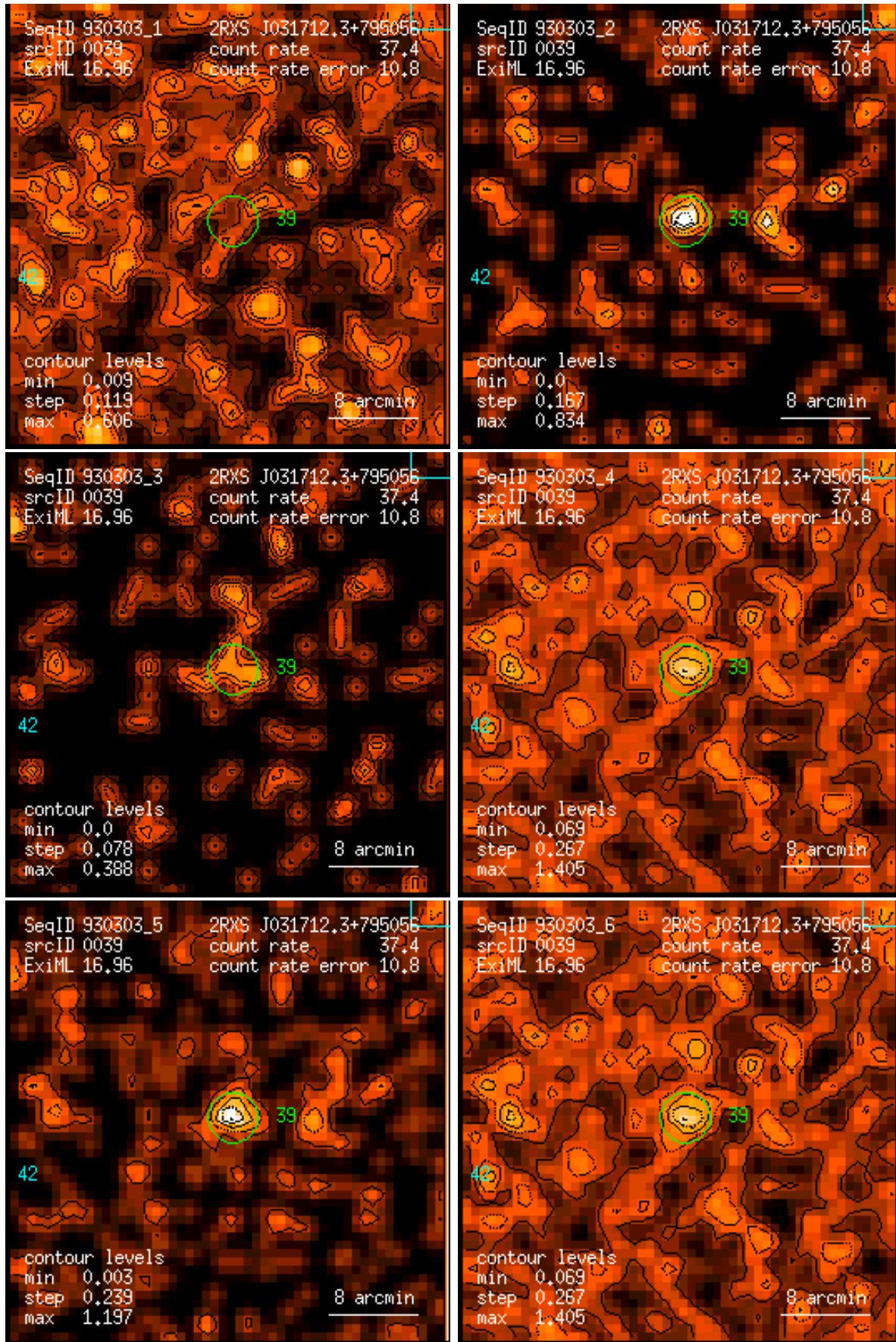
Figure 39: RASS 930303: detection 0039: band rate images, Gaussian filter: (1) PSPC channels 11 – 41, (2) 52 – 90, (3) 91 – 201, (4) 11 – 235, (5) 52 – 201, (6) 11 – 201. Broad band rates in counts/ks. Band rate contour levels in counts/ks/arcmin 2 .
