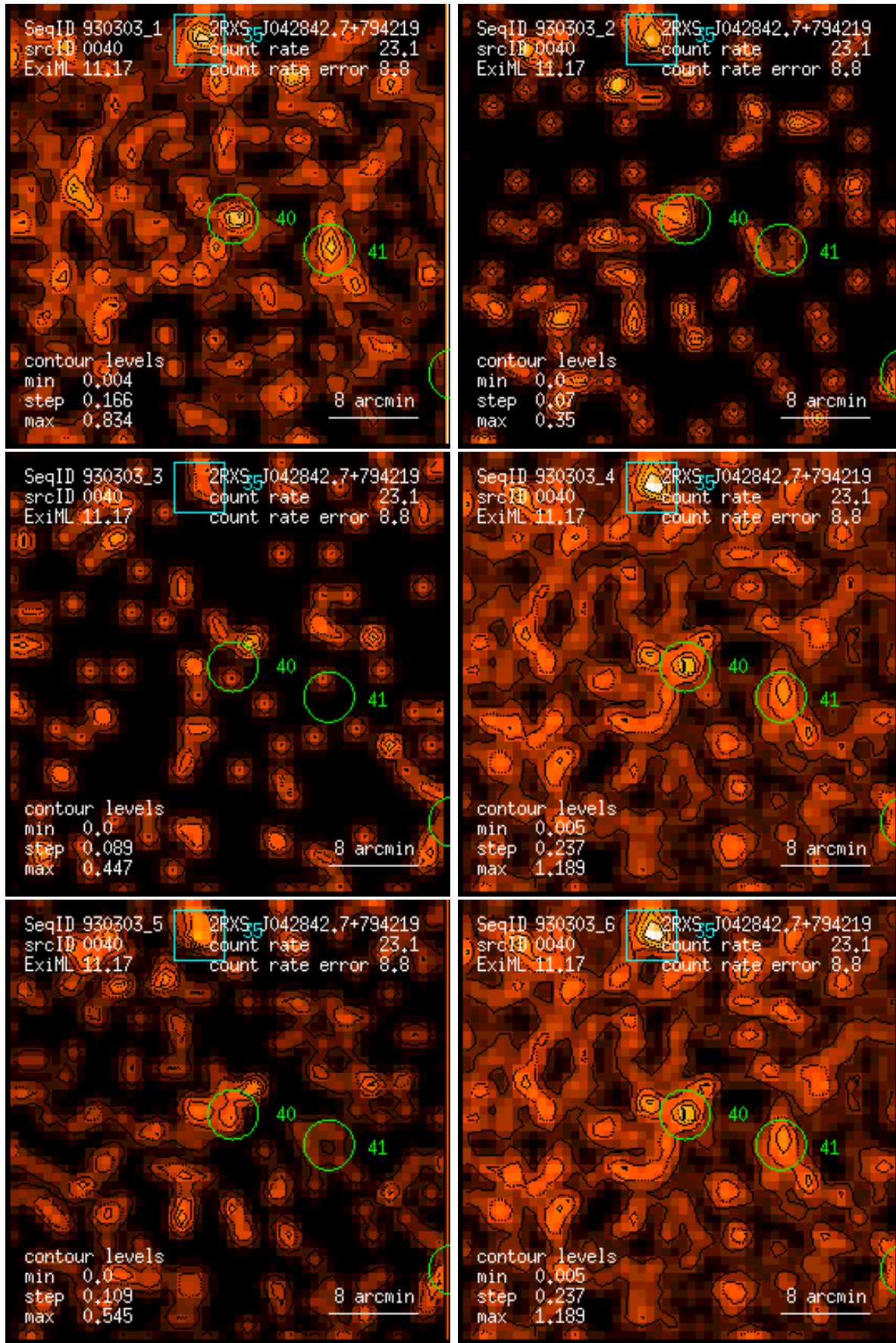
Figure 40: RASS 930303: detection 0040: band rate images, Gaussian filter: (1) PSPC channels 11 – 41, (2) 52 – 90, (3) 91 – 201, (4) 11 – 235, (5) 52 – 201, (6) 11 – 201. Broad band rates in counts/ks. Band rate contour levels in counts/ks/arcmin 2 .
