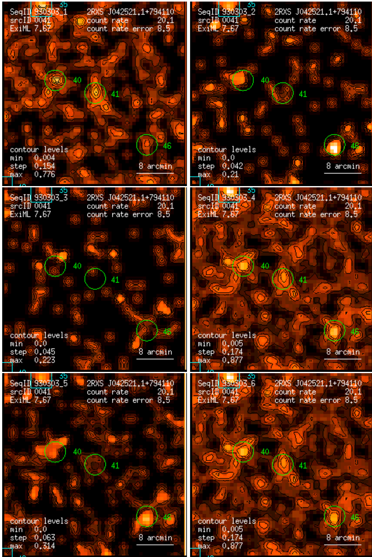
Figure 41: RASS 930303: detection 0041: band rate images, Gaussian filter: (1) PSPC channels 11 – 41, (2) 52 – 90, (3) 91 – 201, (4) 11 – 235, (5) 52 – 201, (6) 11 – 201. Broad band rates in counts/ks. Band rate contour levels in counts/ks/arcmin 2 .
