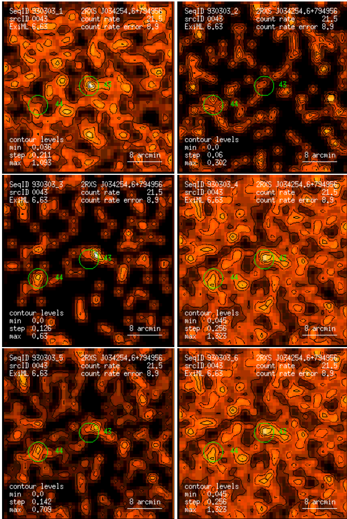
Figure 43: RASS 930303: detection 0043: band rate images, Gaussian filter: (1) PSPC channels 11 – 41, (2) 52 – 90, (3) 91 – 201, (4) 11 – 235, (5) 52 – 201, (6) 11 – 201. Broad band rates in counts/ks. Band rate contour levels in counts/ks/arcmin 2 .
