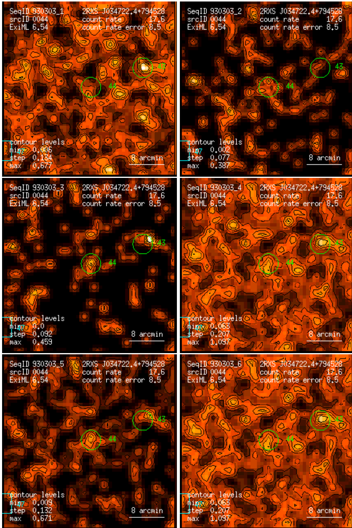
Figure 44: RASS 930303: detection 0044: band rate images, Gaussian filter: (1) PSPC channels 11 – 41, (2) 52 – 90, (3) 91 – 201, (4) 11 – 235, (5) 52 – 201, (6) 11 – 201. Broad band rates in counts/ks. Band rate contour levels in counts/ks/arcmin 2 .
