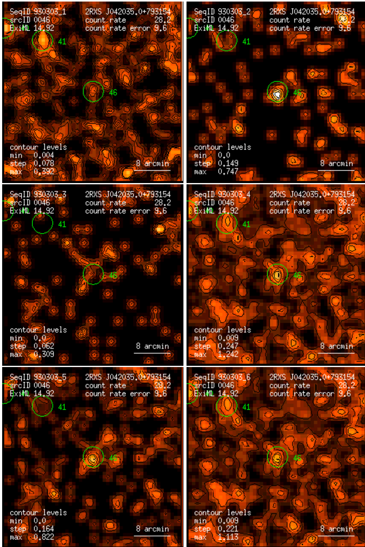
Figure 46: RASS 930303: detection 0046: band rate images, Gaussian filter: (1) PSPC channels 11 – 41, (2) 52 – 90, (3) 91 – 201, (4) 11 – 235, (5) 52 – 201, (6) 11 – 201. Broad band rates in counts/ks. Band rate contour levels in counts/ks/arcmin 2 .
