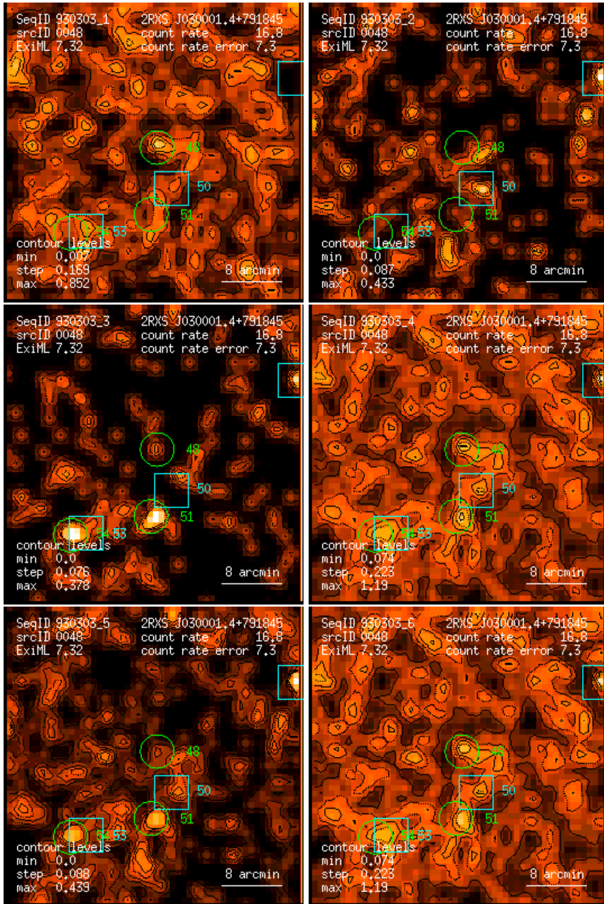
Figure 48: RASS 930303: detection 0048: band rate images, Gaussian filter: (1) PSPC channels 11 – 41, (2) 52 – 90, (3) 91 – 201, (4) 11 – 235, (5) 52 – 201, (6) 11 – 201. Broad band rates in counts/ks. Band rate contour levels in counts/ks/arcmin 2 .
