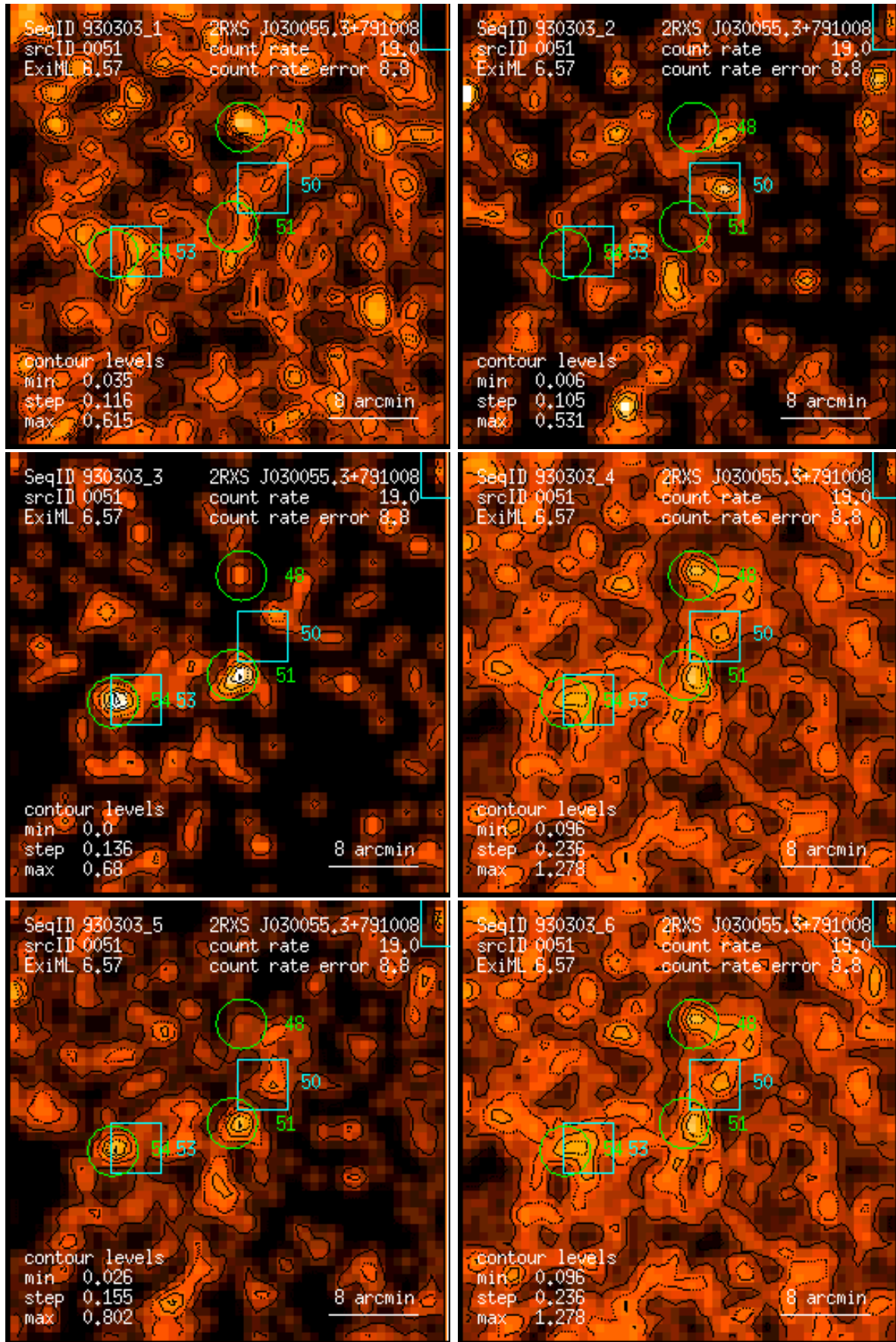
Figure 51: RASS 930303: detection 0051: band rate images, Gaussian filter: (1) PSPC channels 11 – 41, (2) 52 – 90, (3) 91 – 201, (4) 11 – 235, (5) 52 – 201, (6) 11 – 201. Broad band rates in counts/ks. Band rate contour levels in counts/ks/arcmin 2 .
