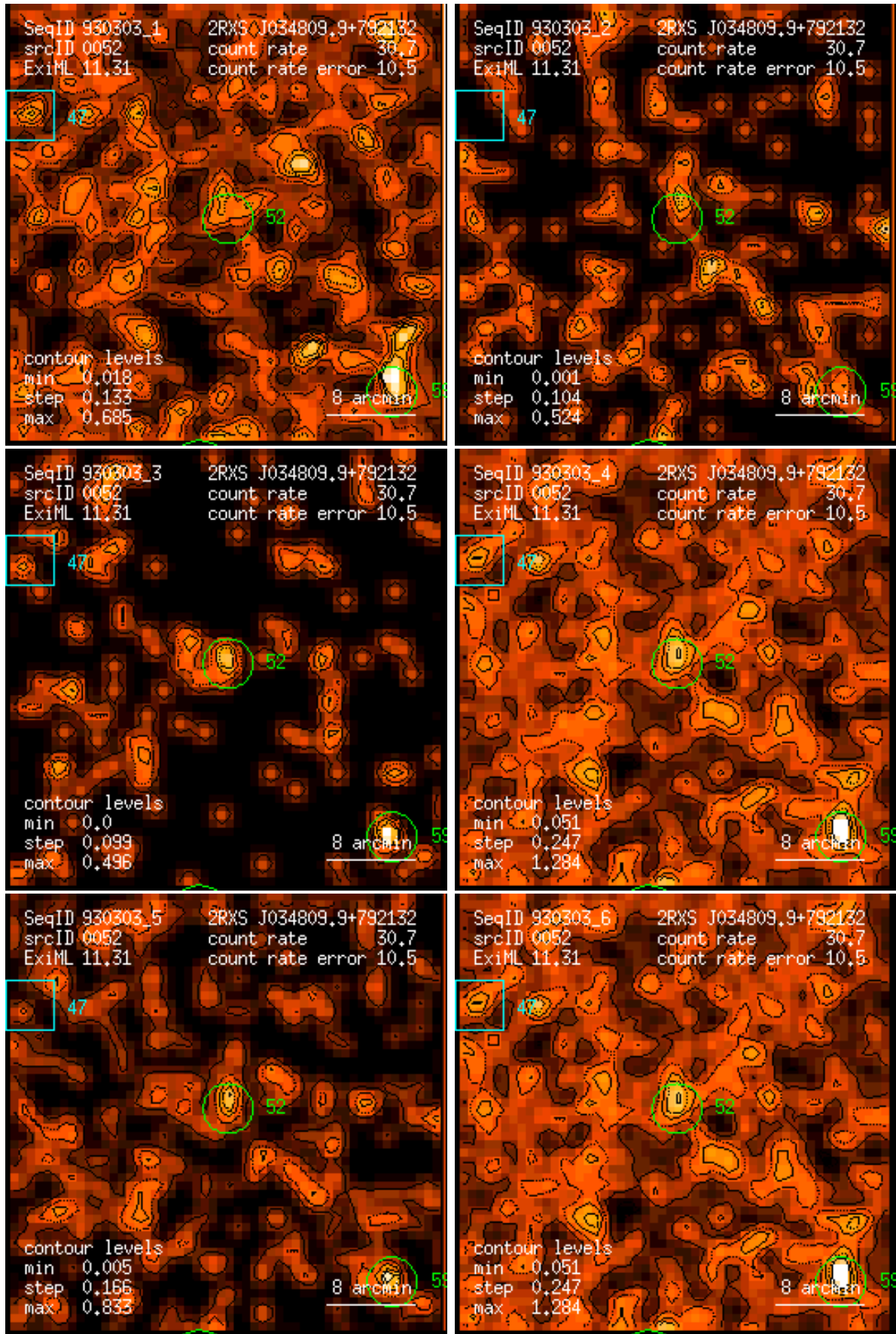
Figure 52: RASS 930303: detection 0052: band rate images, Gaussian filter: (1) PSPC channels 11 – 41, (2) 52 – 90, (3) 91 – 201, (4) 11 – 235, (5) 52 – 201, (6) 11 – 201. Broad band rates in counts/ks. Band rate contour levels in counts/ks/arcmin 2 .
