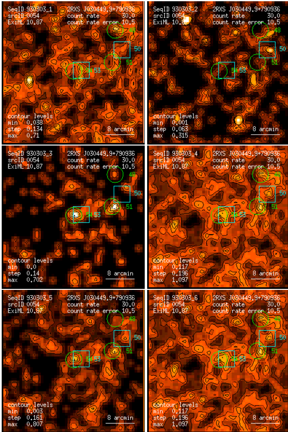
Figure 54: RASS 930303: detection 0054: band rate images, Gaussian filter: (1) PSPC channels 11 – 41, (2) 52 – 90, (3) 91 – 201, (4) 11 – 235, (5) 52 – 201, (6) 11 – 201. Broad band rates in counts/ks. Band rate contour levels in counts/ks/arcmin 2 .
