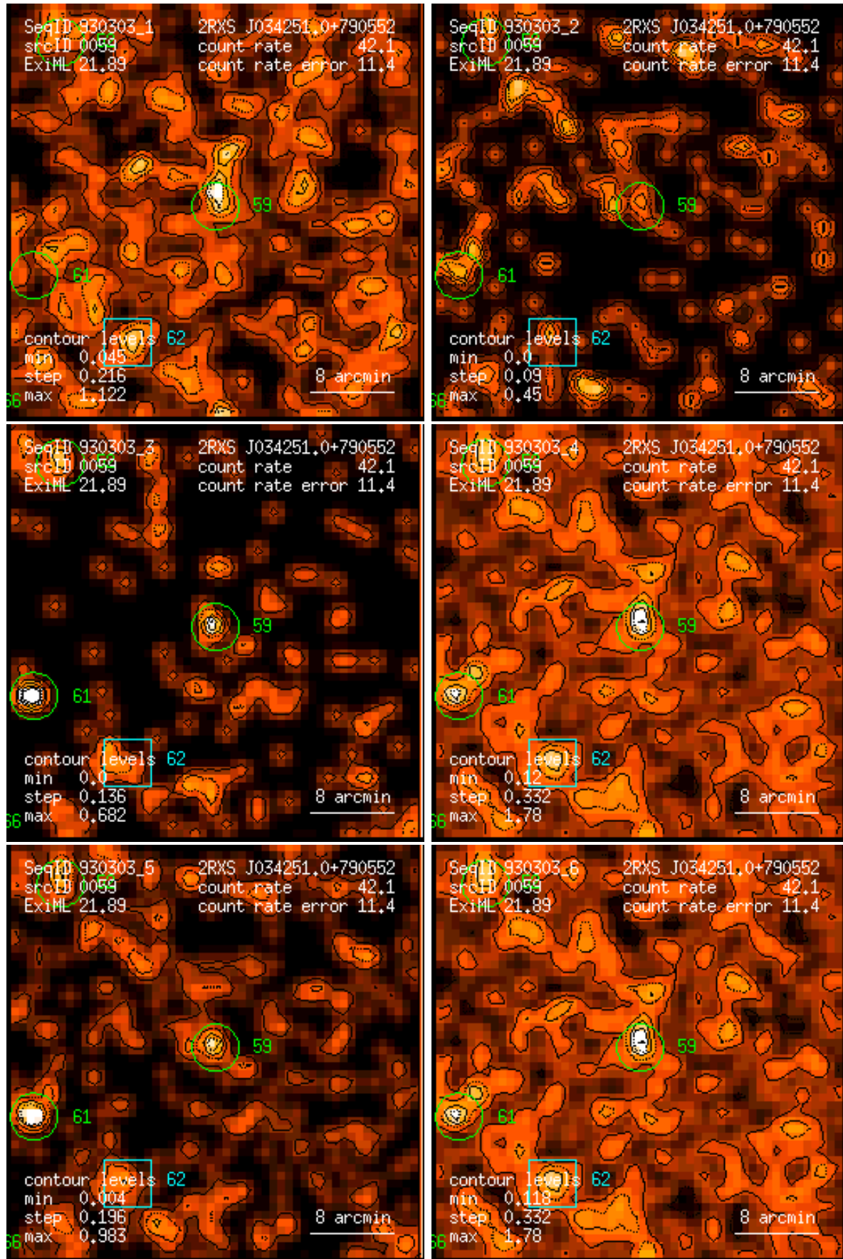
Figure 59: RASS 930303: detection 0059: band rate images, Gaussian filter: (1) PSPC channels 11 – 41, (2) 52 – 90, (3) 91 – 201, (4) 11 – 235, (5) 52 – 201, (6) 11 – 201. Broad band rates in counts/ks. Band rate contour levels in counts/ks/arcmin 2 .
