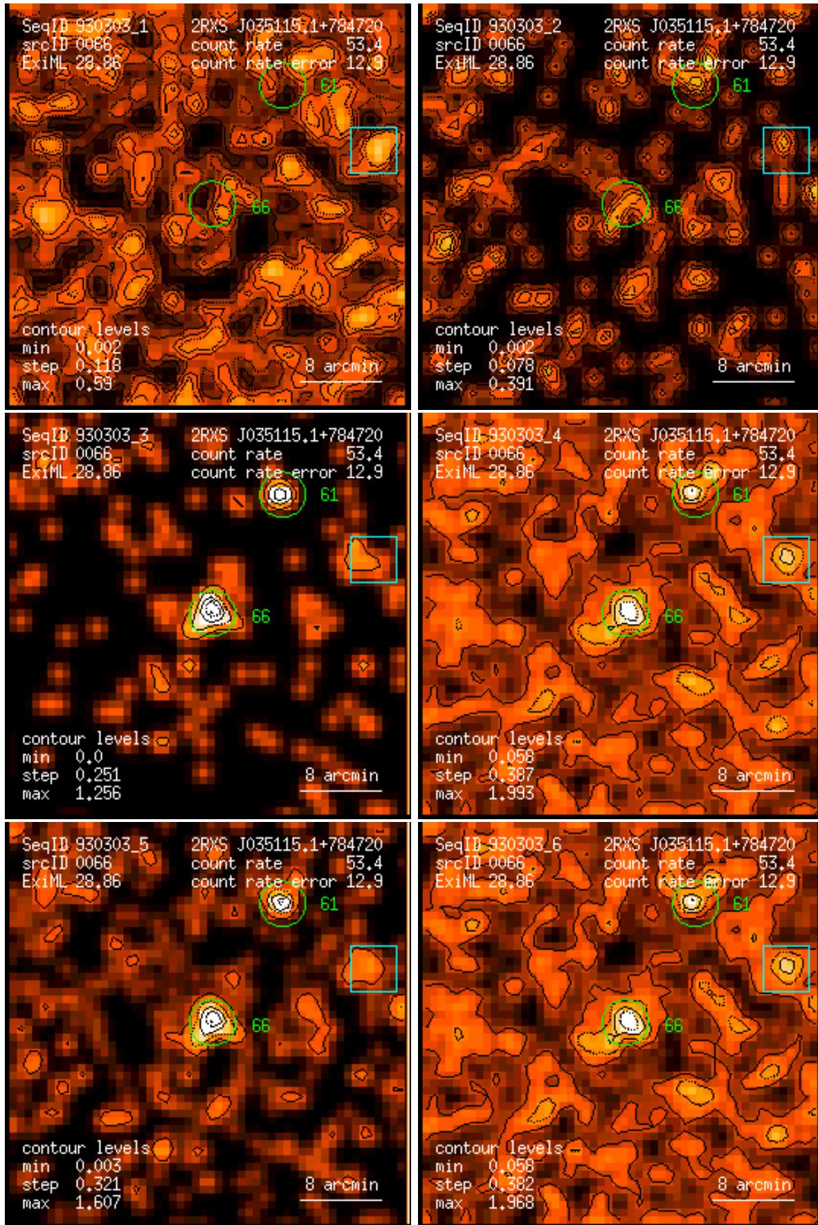
Figure 66: RASS 930303: detection 0066: band rate images, Gaussian filter: (1) PSPC channels 11 – 41, (2) 52 – 90, (3) 91 – 201, (4) 11 – 235, (5) 52 – 201, (6) 11 – 201. Broad band rates in counts/ks. Band rate contour levels in counts/ks/arcmin 2 .
