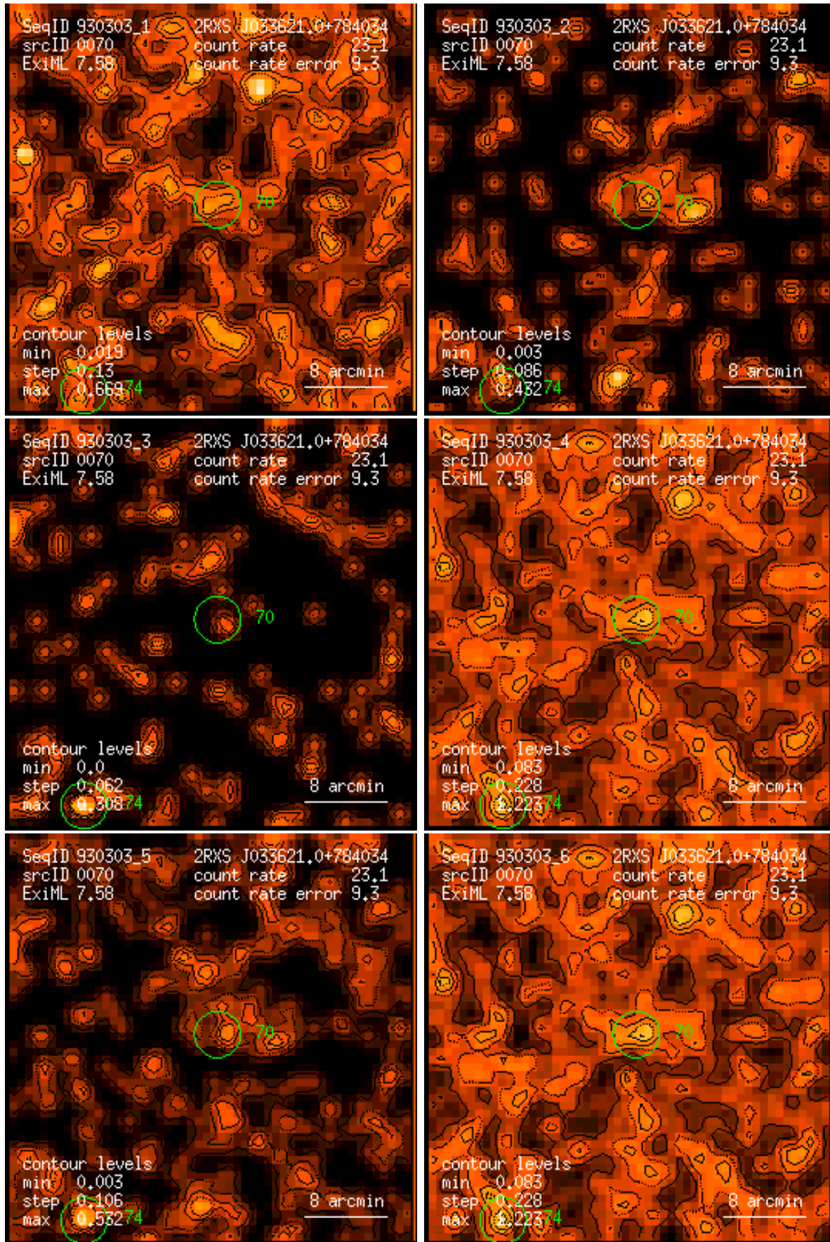
Figure 70: RASS 930303: detection 0070: band rate images, Gaussian filter: (1) PSPC channels 11 – 41, (2) 52 – 90, (3) 91 – 201, (4) 11 – 235, (5) 52 – 201, (6) 11 – 201. Broad band rates in counts/ks. Band rate contour levels in counts/ks/arcmin 2 .
