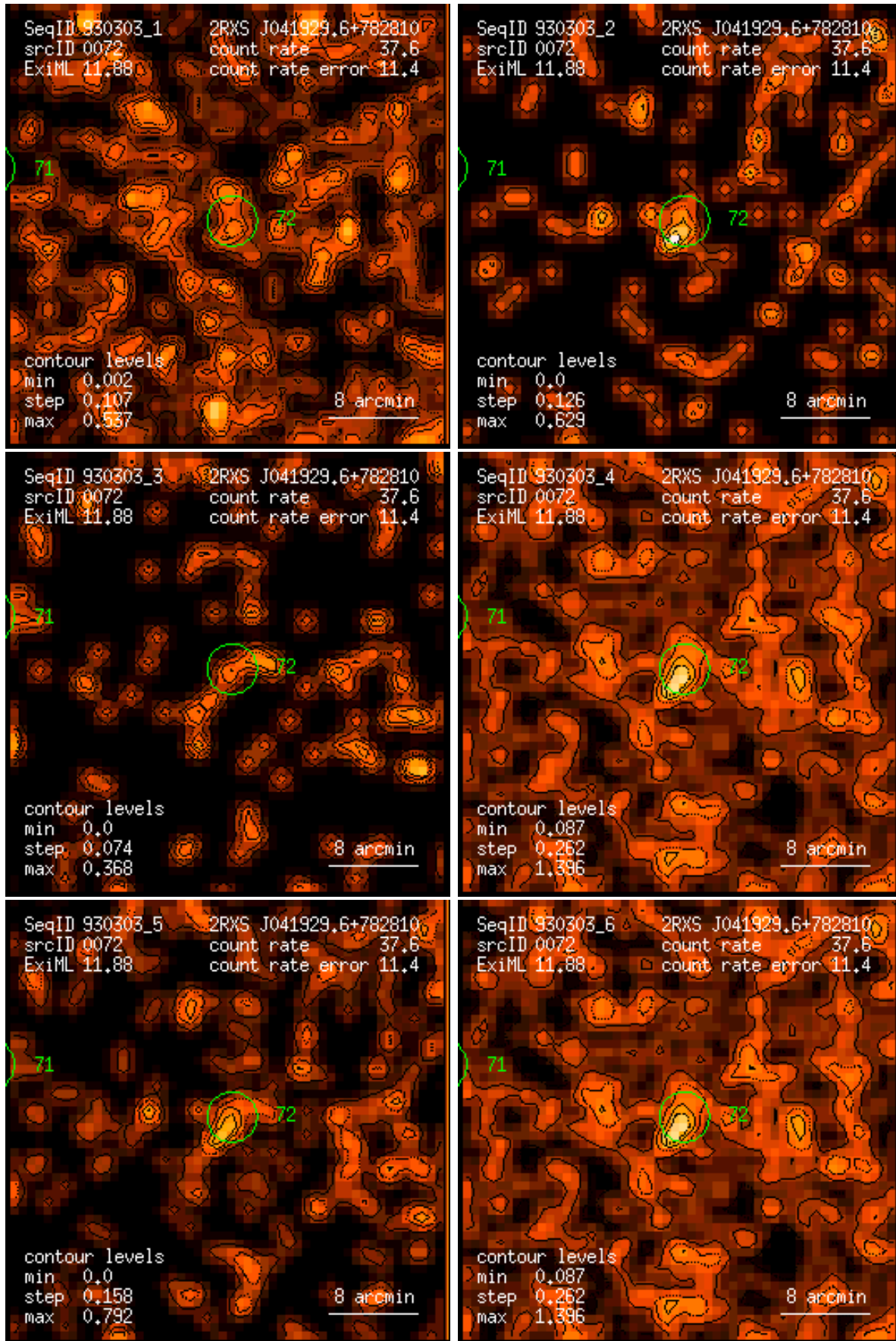
Figure 72: RASS 930303: detection 0072: band rate images, Gaussian filter: (1) PSPC channels 11 – 41, (2) 52 – 90, (3) 91 – 201, (4) 11 – 235, (5) 52 – 201, (6) 11 – 201. Broad band rates in counts/ks. Band rate contour levels in counts/ks/arcmin 2 .
