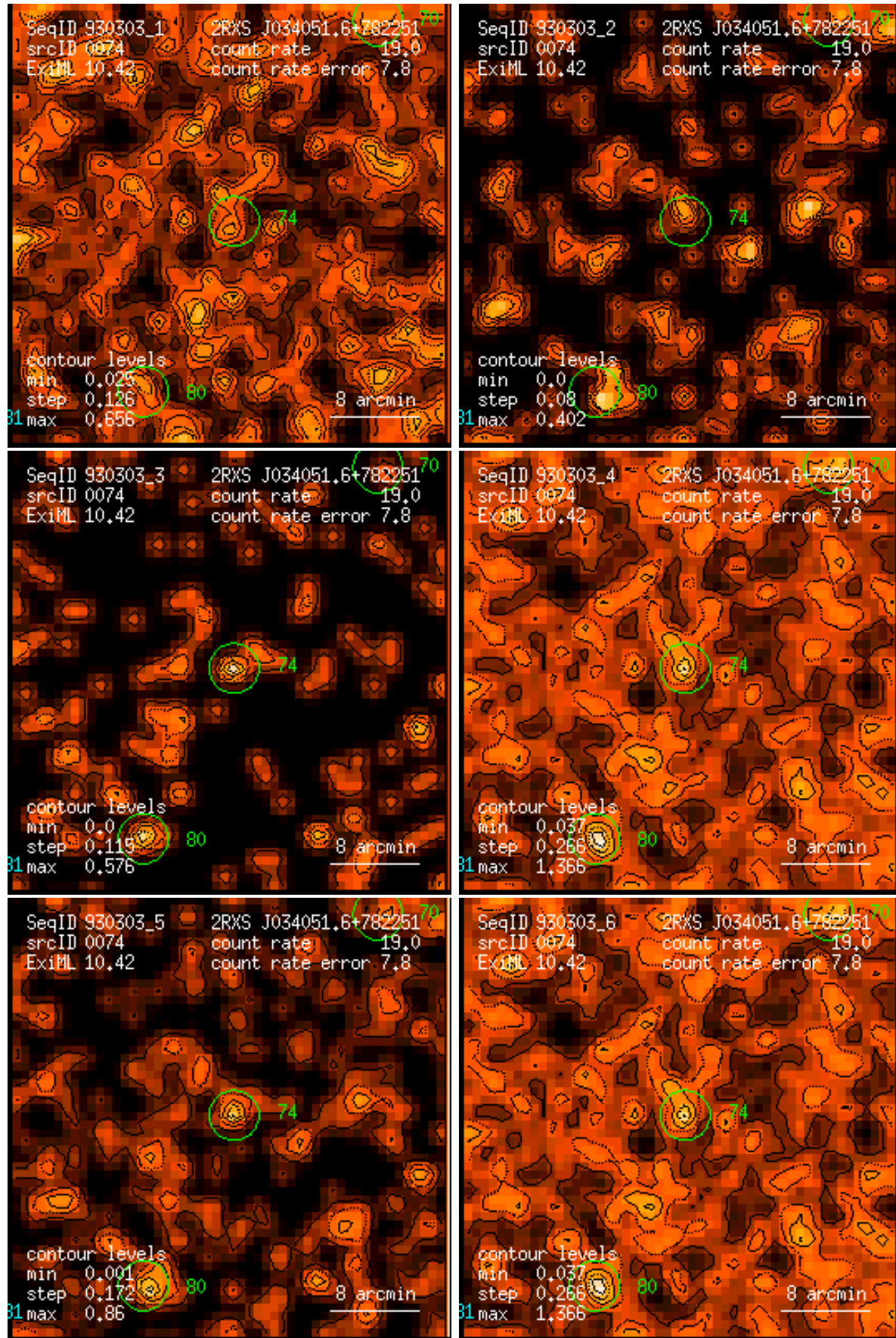
Figure 74: RASS 930303: detection 0074: band rate images, Gaussian filter: (1) PSPC channels 11 – 41, (2) 52 – 90, (3) 91 – 201, (4) 11 – 235, (5) 52 – 201, (6) 11 – 201. Broad band rates in counts/ks. Band rate contour levels in counts/ks/arcmin 2 .
